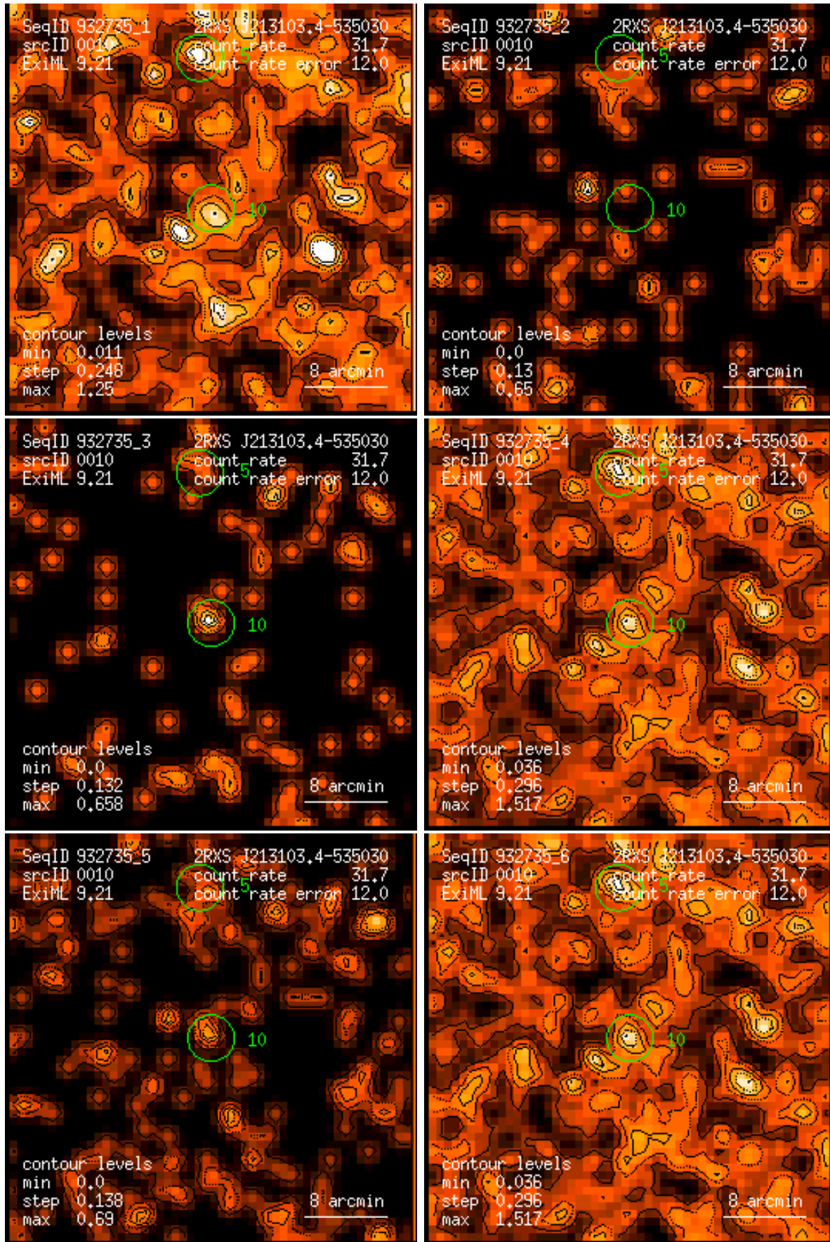
Figure 10: RASS 932735: detection 0010: band rate images, Gaussian filter: (1) PSPC channels 11 – 41, (2) 52 – 90, (3) 91 – 201, (4) 11 – 235, (5) 52 – 201, (6) 11 – 201. Broad band rates in counts/ks. Band rate contour levels in counts/ks/arcmin 2 .
