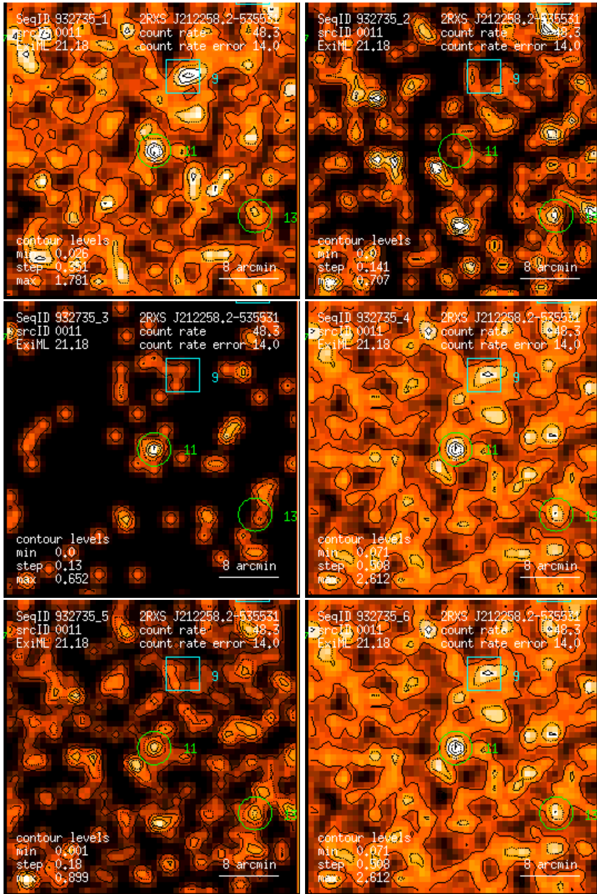
Figure 11: RASS 932735: detection 0011: band rate images, Gaussian filter: (1) PSPC channels 11 – 41, (2) 52 – 90, (3) 91 – 201, (4) 11 – 235, (5) 52 – 201, (6) 11 – 201. Broad band rates in counts/ks. Band rate contour levels in counts/ks/arcmin 2 .
