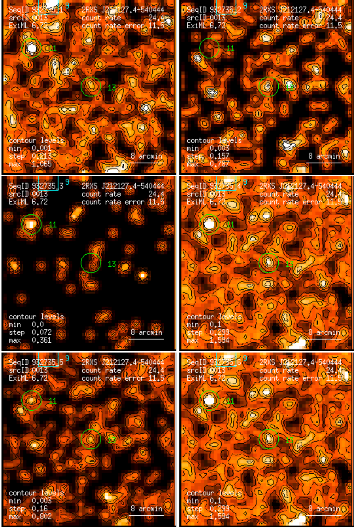
Figure 13: RASS 932735: detection 0013: band rate images, Gaussian filter: (1) PSPC channels 11 – 41, (2) 52 – 90, (3) 91 – 201, (4) 11 – 235, (5) 52 – 201, (6) 11 – 201. Broad band rates in counts/ks. Band rate contour levels in counts/ks/arcmin 2 .
