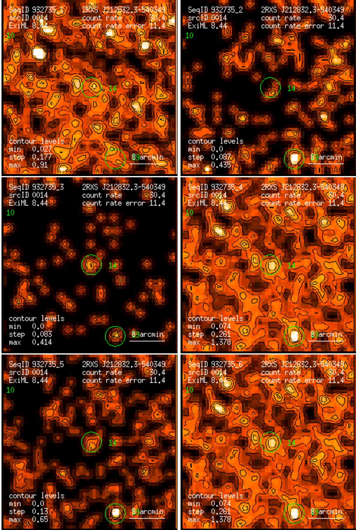
Figure 14: RASS 932735: detection 0014: band rate images, Gaussian filter: (1) PSPC channels 11 – 41, (2) 52 – 90, (3) 91 – 201, (4) 11 – 235, (5) 52 – 201, (6) 11 – 201. Broad band rates in counts/ks. Band rate contour levels in counts/ks/arcmin 2 .
