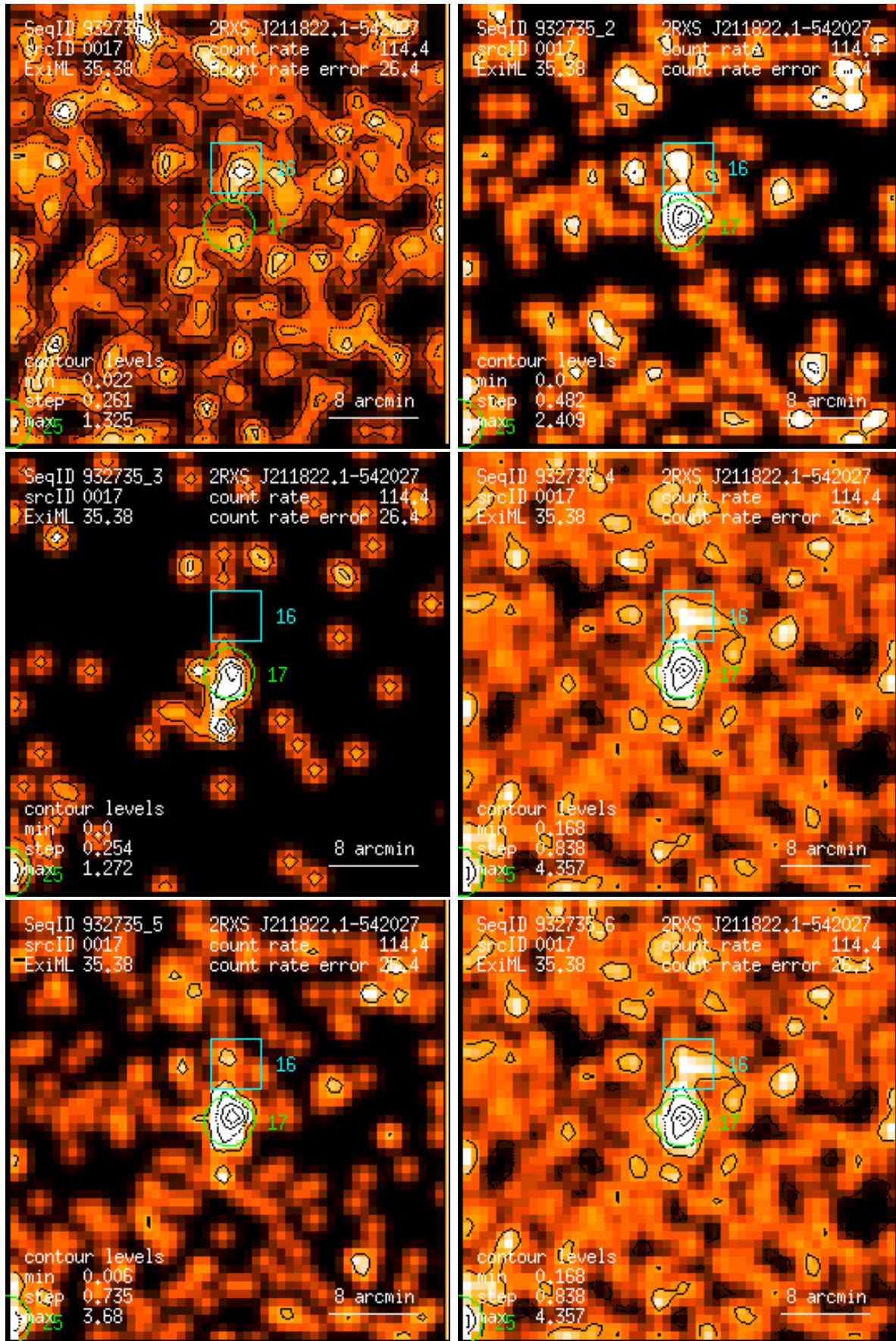
Figure 17: RASS 932735: detection 0017: band rate images, Gaussian filter: (1) PSPC channels 11 – 41, (2) 52 – 90, (3) 91 – 201, (4) 11 – 235, (5) 52 – 201, (6) 11 – 201. Broad band rates in counts/ks. Band rate contour levels in counts/ks/arcmin 2 .
