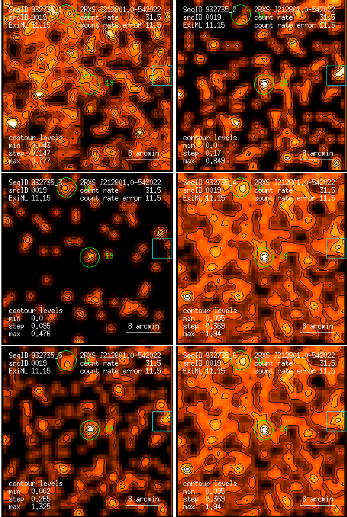
Figure 19: RASS 932735: detection 0019: band rate images, Gaussian filter: (1) PSPC channels 11 – 41, (2) 52 – 90, (3) 91 – 201, (4) 11 – 235, (5) 52 – 201, (6) 11 – 201. Broad band rates in counts/ks. Band rate contour levels in counts/ks/arcmin 2 .
