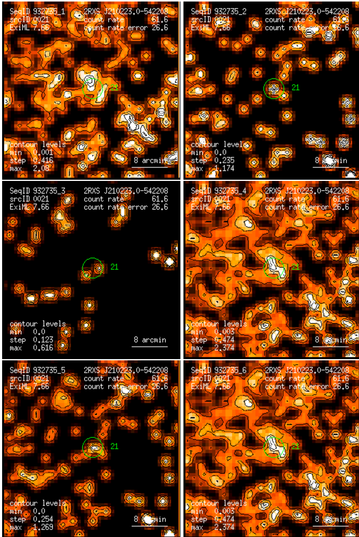
Figure 21: RASS 932735: detection 0021: band rate images, Gaussian filter: (1) PSPC channels 11 – 41, (2) 52 – 90, (3) 91 – 201, (4) 11 – 235, (5) 52 – 201, (6) 11 – 201. Broad band rates in counts/ks. Band rate contour levels in counts/ks/arcmin 2 .
