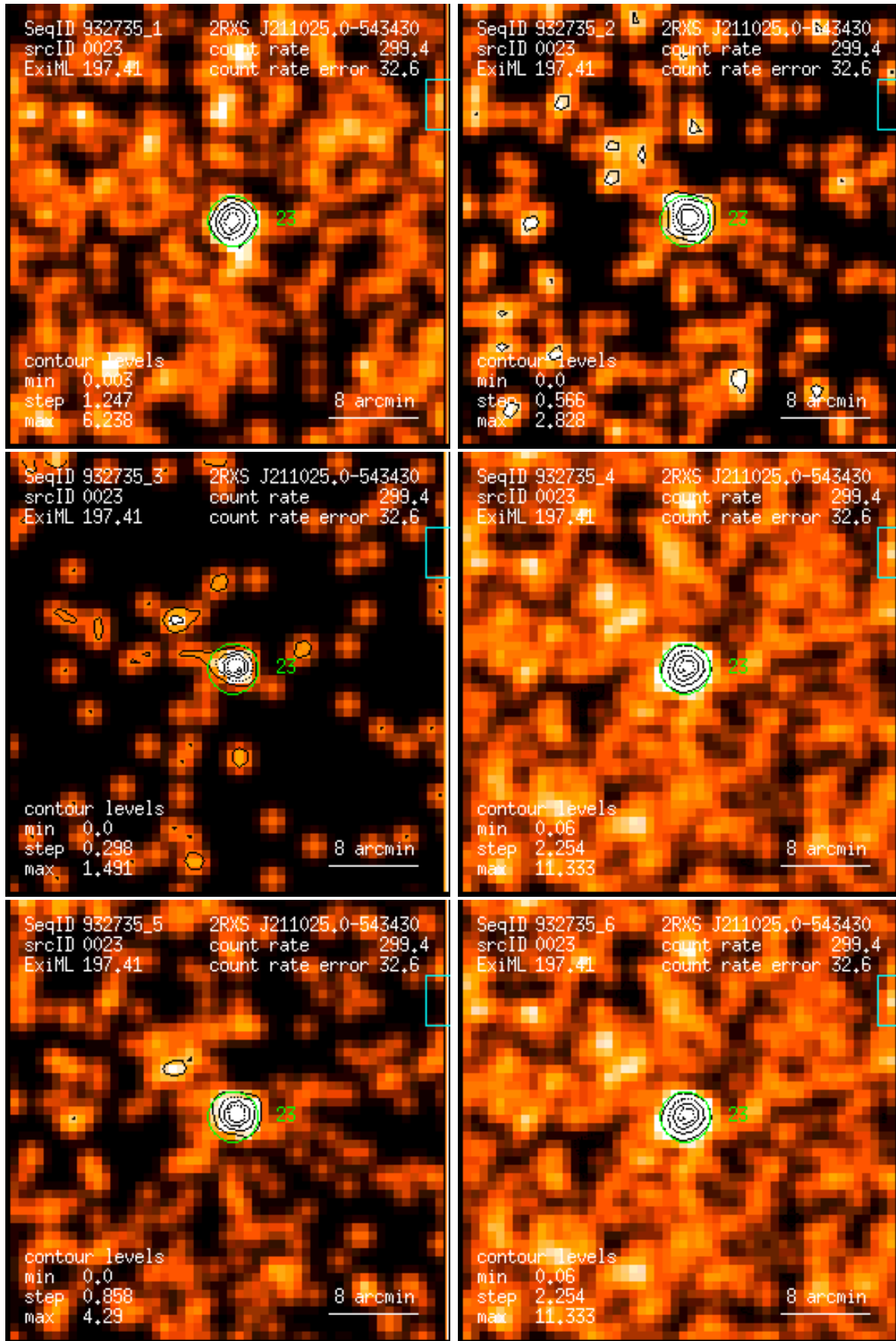
Figure 23: RASS 932735: detection 0023: band rate images, Gaussian filter: (1) PSPC channels 11 – 41, (2) 52 – 90, (3) 91 – 201, (4) 11 – 235, (5) 52 – 201, (6) 11 – 201. Broad band rates in counts/ks. Band rate contour levels in counts/ks/arcmin 2 .
