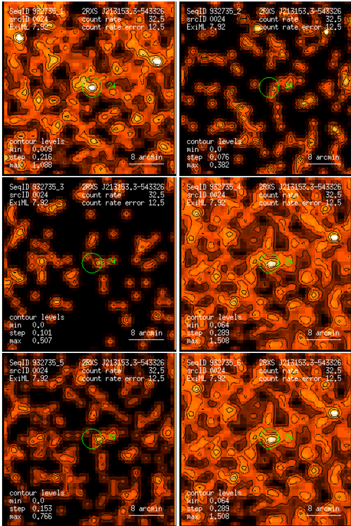
Figure 24: RASS 932735: detection 0024: band rate images, Gaussian filter: (1) PSPC channels 11 – 41, (2) 52 – 90, (3) 91 – 201, (4) 11 – 235, (5) 52 – 201, (6) 11 – 201. Broad band rates in counts/ks. Band rate contour levels in counts/ks/arcmin 2 .
