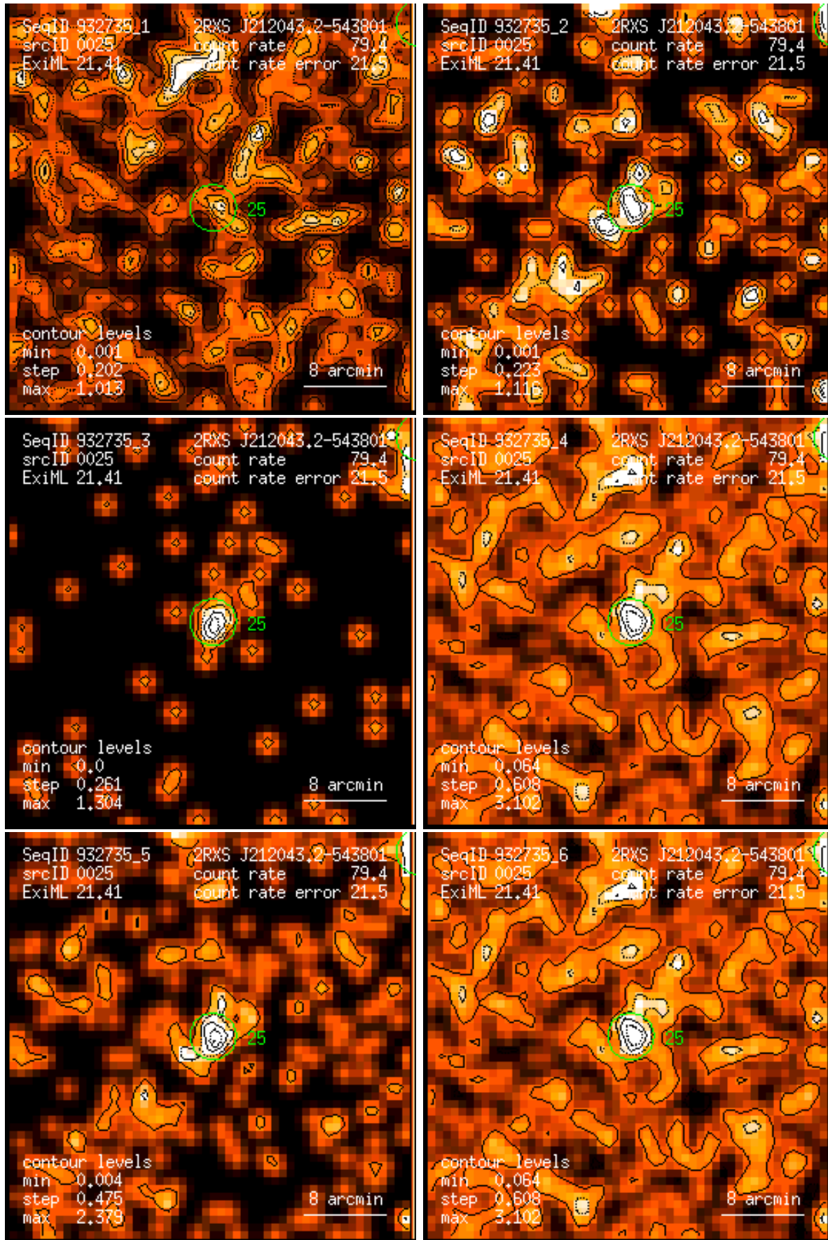
Figure 25: RASS 932735: detection 0025: band rate images, Gaussian filter: (1) PSPC channels 11 – 41, (2) 52 – 90, (3) 91 – 201, (4) 11 – 235, (5) 52 – 201, (6) 11 – 201. Broad band rates in counts/ks. Band rate contour levels in counts/ks/arcmin 2 .
