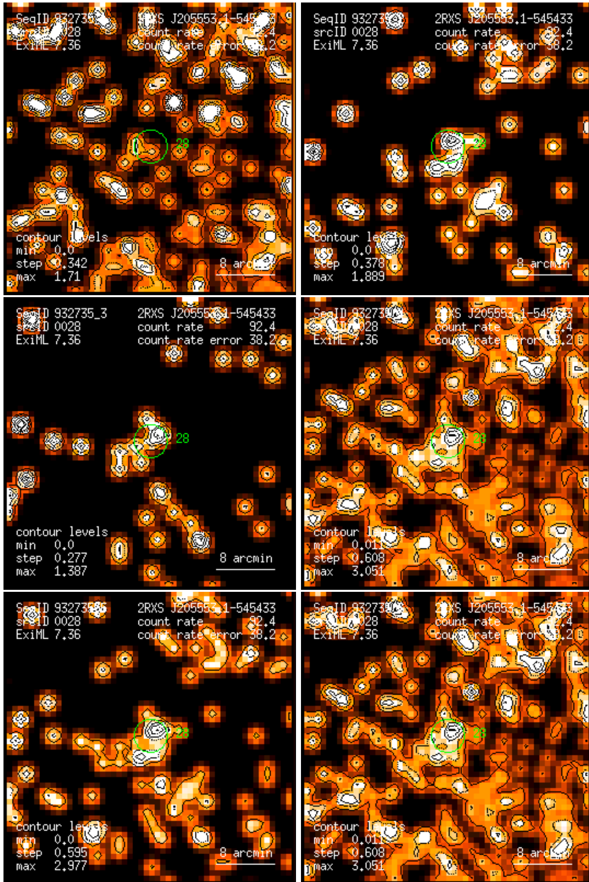
Figure 28: RASS 932735: detection 0028: band rate images, Gaussian filter: (1) PSPC channels 11 – 41, (2) 52 – 90, (3) 91 – 201, (4) 11 – 235, (5) 52 – 201, (6) 11 – 201. Broad band rates in counts/ks. Band rate contour levels in counts/ks/arcmin 2 .
