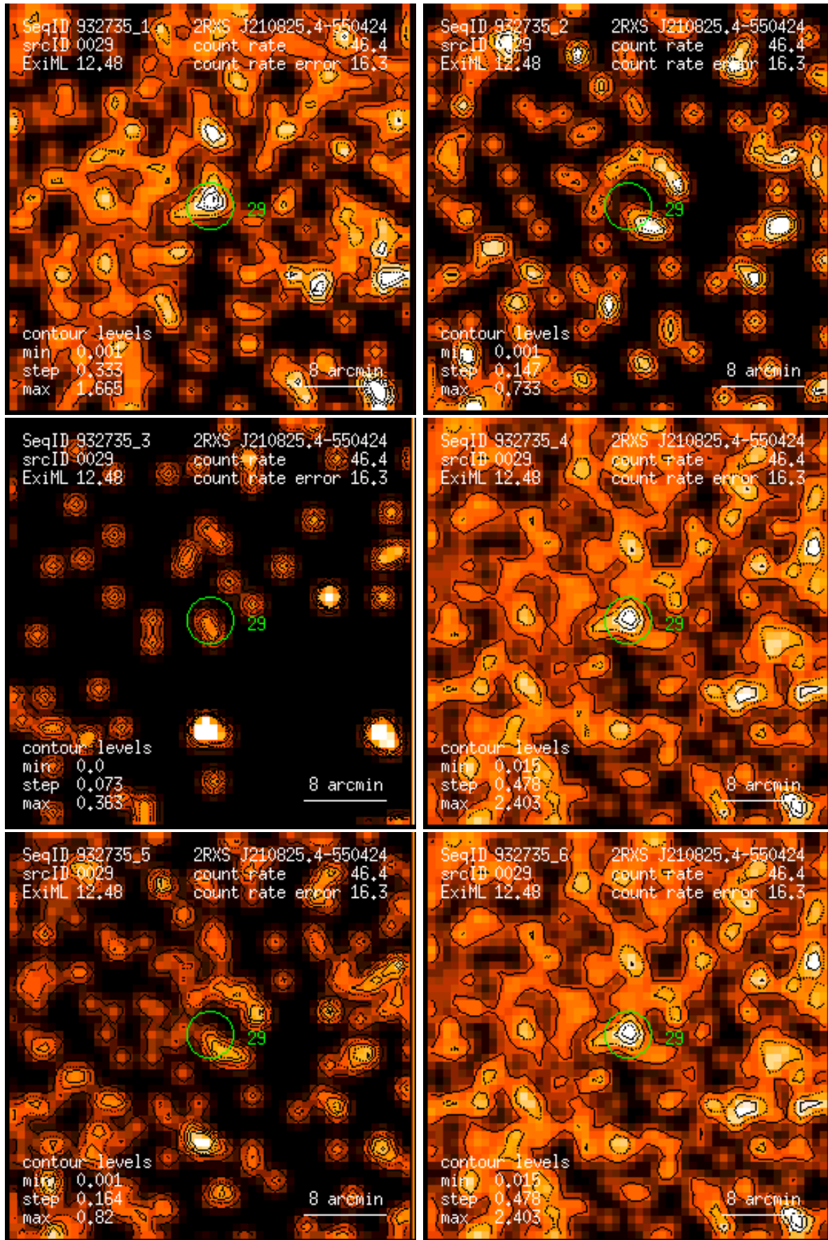
Figure 29: RASS 932735: detection 0029: band rate images, Gaussian filter: (1) PSPC channels 11 – 41, (2) 52 – 90, (3) 91 – 201, (4) 11 – 235, (5) 52 – 201, (6) 11 – 201. Broad band rates in counts/ks. Band rate contour levels in counts/ks/arcmin 2 .
