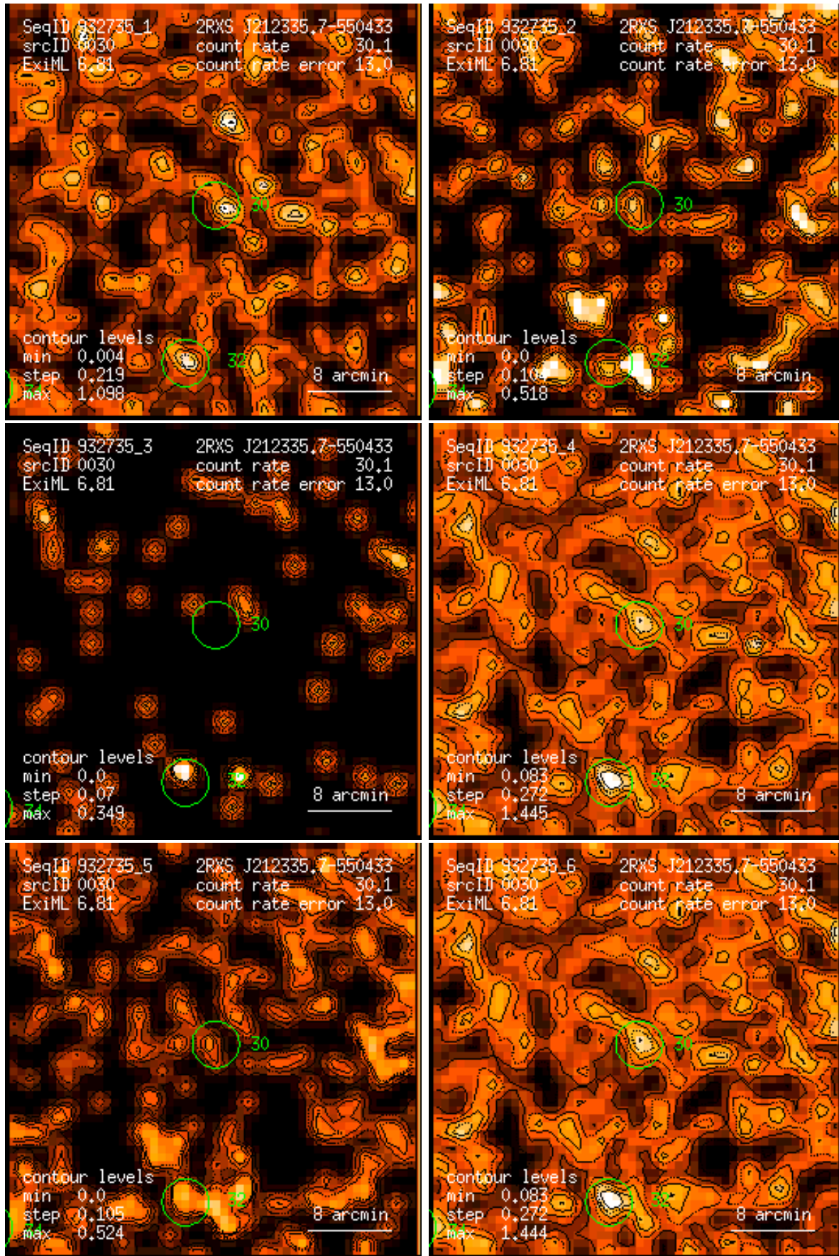
Figure 30: RASS 932735: detection 0030: band rate images, Gaussian filter: (1) PSPC channels 11 – 41, (2) 52 – 90, (3) 91 – 201, (4) 11 – 235, (5) 52 – 201, (6) 11 – 201. Broad band rates in counts/ks. Band rate contour levels in counts/ks/arcmin 2 .
