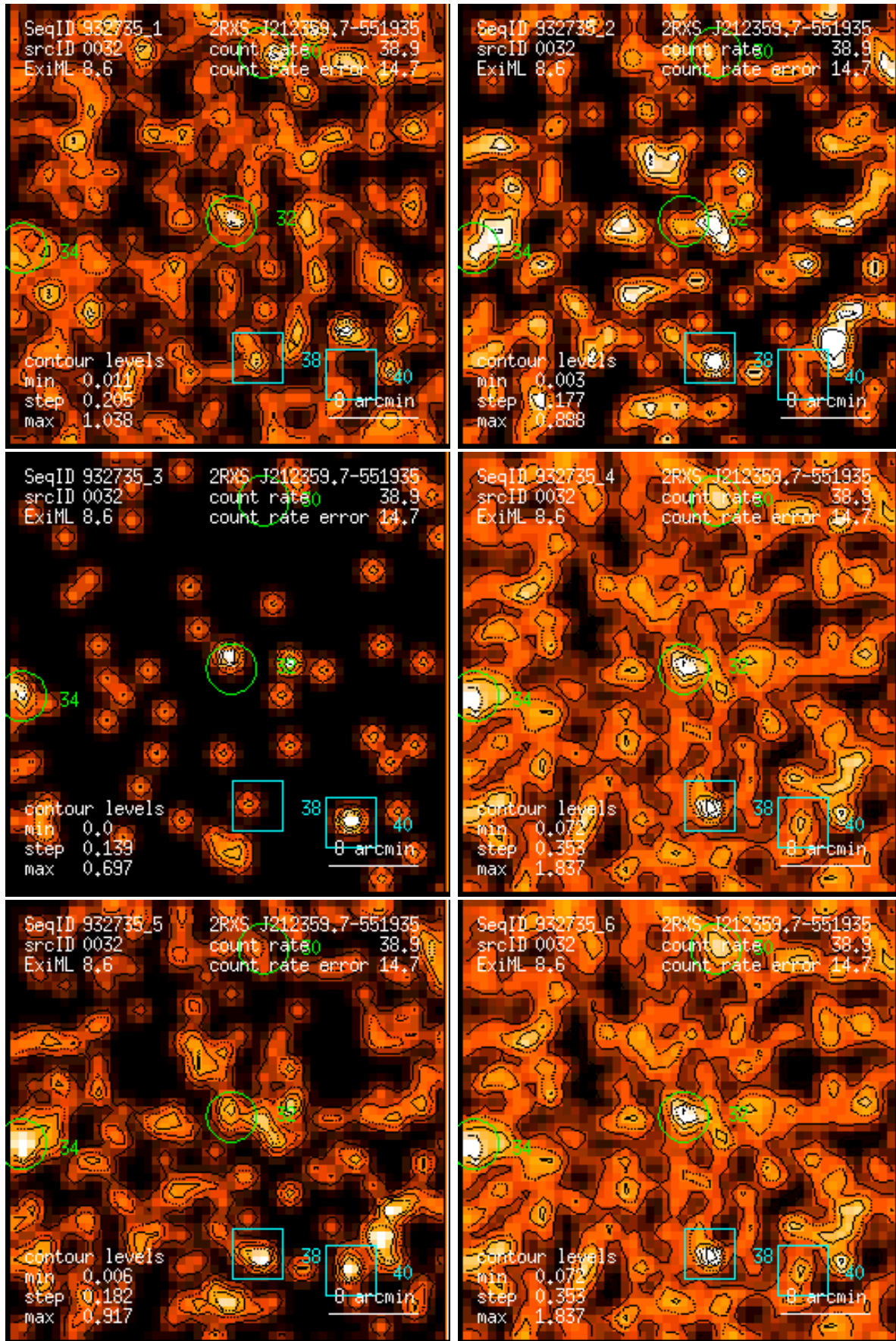
Figure 32: RASS 932735: detection 0032: band rate images, Gaussian filter: (1) PSPC channels 11 – 41, (2) 52 – 90, (3) 91 – 201, (4) 11 – 235, (5) 52 – 201, (6) 11 – 201. Broad band rates in counts/ks. Band rate contour levels in counts/ks/arcmin 2 .
