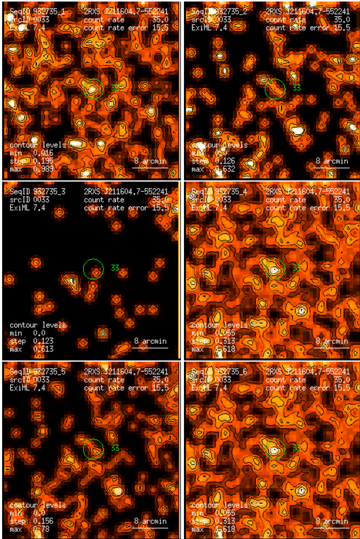
Figure 33: RASS 932735: detection 0033: band rate images, Gaussian filter: (1) PSPC channels 11 – 41, (2) 52 – 90, (3) 91 – 201, (4) 11 – 235, (5) 52 – 201, (6) 11 – 201. Broad band rates in counts/ks. Band rate contour levels in counts/ks/arcmin 2 .
