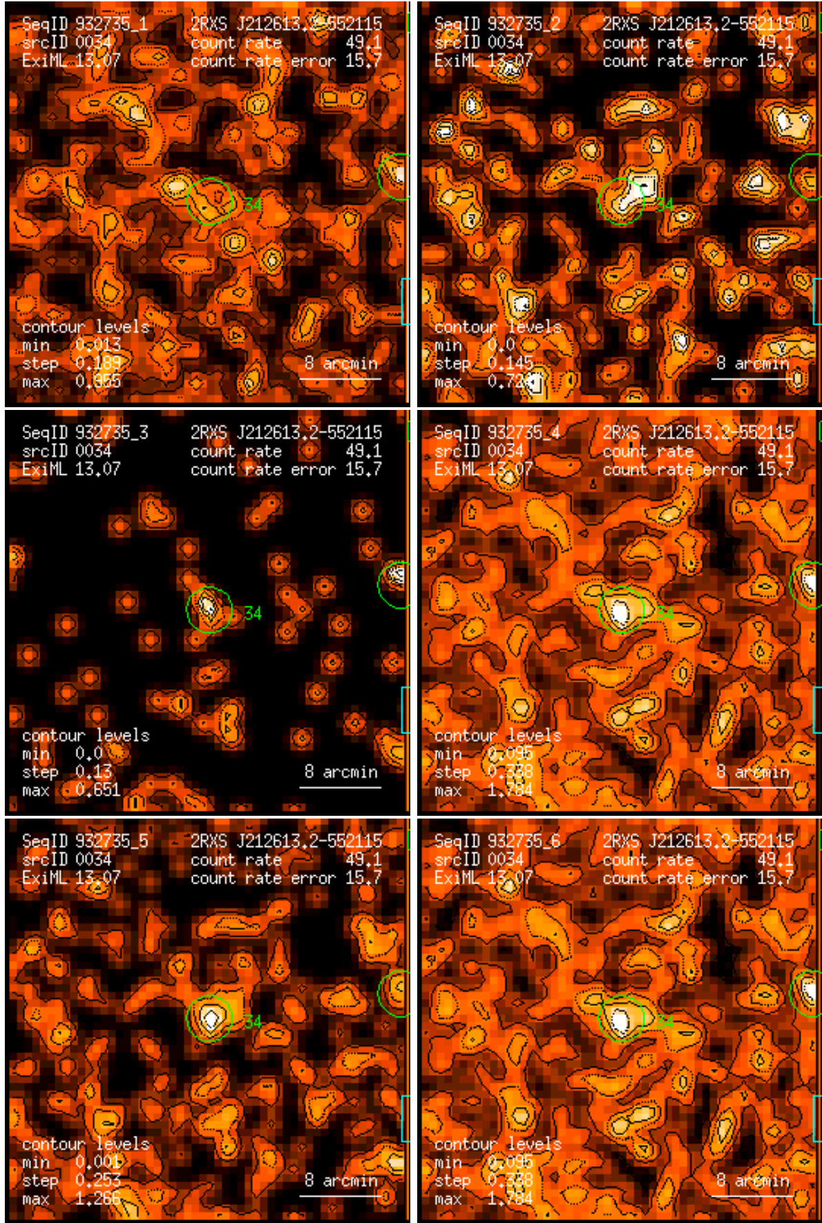
Figure 34: RASS 932735: detection 0034: band rate images, Gaussian filter: (1) PSPC channels 11 – 41, (2) 52 – 90, (3) 91 – 201, (4) 11 – 235, (5) 52 – 201, (6) 11 – 201. Broad band rates in counts/ks. Band rate contour levels in counts/ks/arcmin 2 .
