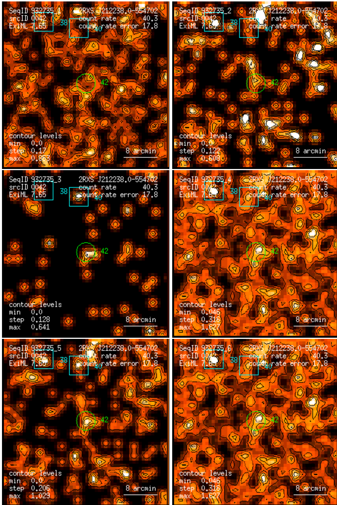
Figure 42: RASS 932735: detection 0042: band rate images, Gaussian filter: (1) PSPC channels 11 – 41, (2) 52 – 90, (3) 91 – 201, (4) 11 – 235, (5) 52 – 201, (6) 11 – 201. Broad band rates in counts/ks. Band rate contour levels in counts/ks/arcmin 2 .
