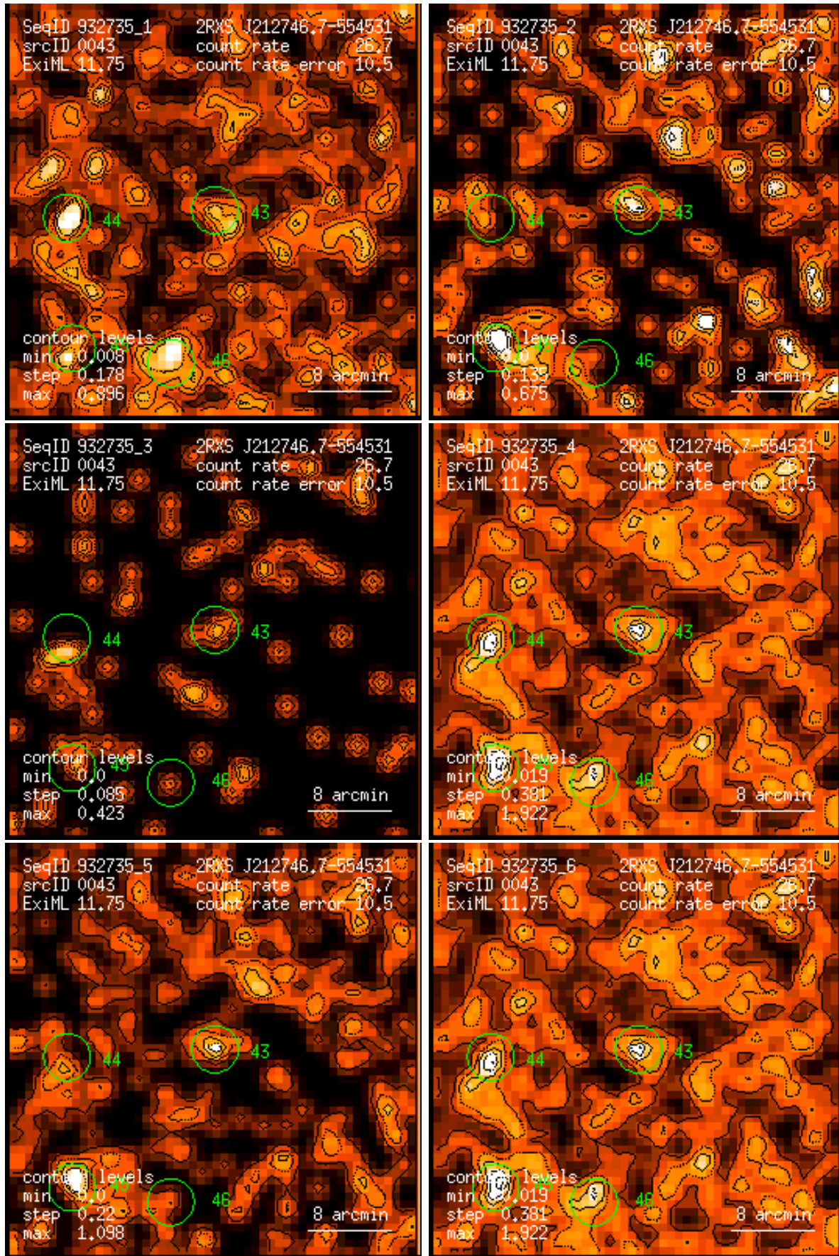
Figure 43: RASS 932735: detection 0043: band rate images, Gaussian filter: (1) PSPC channels 11 – 41, (2) 52 – 90, (3) 91 – 201, (4) 11 – 235, (5) 52 – 201, (6) 11 – 201. Broad band rates in counts/ks. Band rate contour levels in counts/ks/arcmin 2 .
