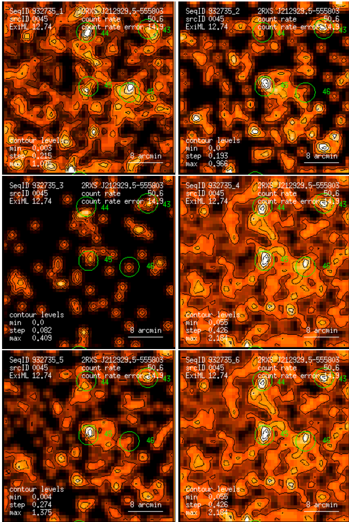
Figure 45: RASS 932735: detection 0045: band rate images, Gaussian filter: (1) PSPC channels 11 – 41, (2) 52 – 90, (3) 91 – 201, (4) 11 – 235, (5) 52 – 201, (6) 11 – 201. Broad band rates in counts/ks. Band rate contour levels in counts/ks/arcmin 2 .
