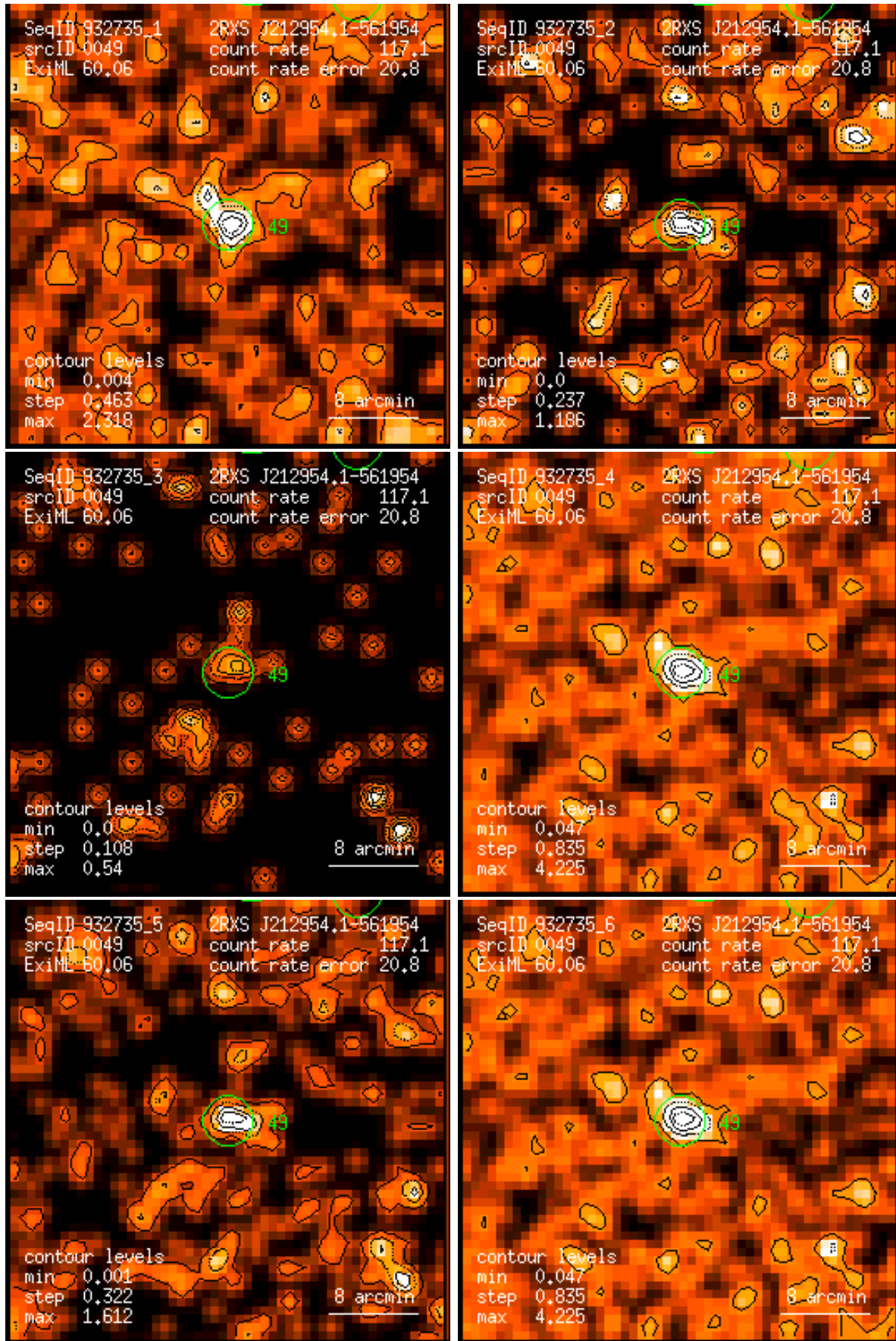
Figure 49: RASS 932735: detection 0049: band rate images, Gaussian filter: (1) PSPC channels 11 – 41, (2) 52 – 90, (3) 91 – 201, (4) 11 – 235, (5) 52 – 201, (6) 11 – 201. Broad band rates in counts/ks. Band rate contour levels in counts/ks/arcmin 2 .
