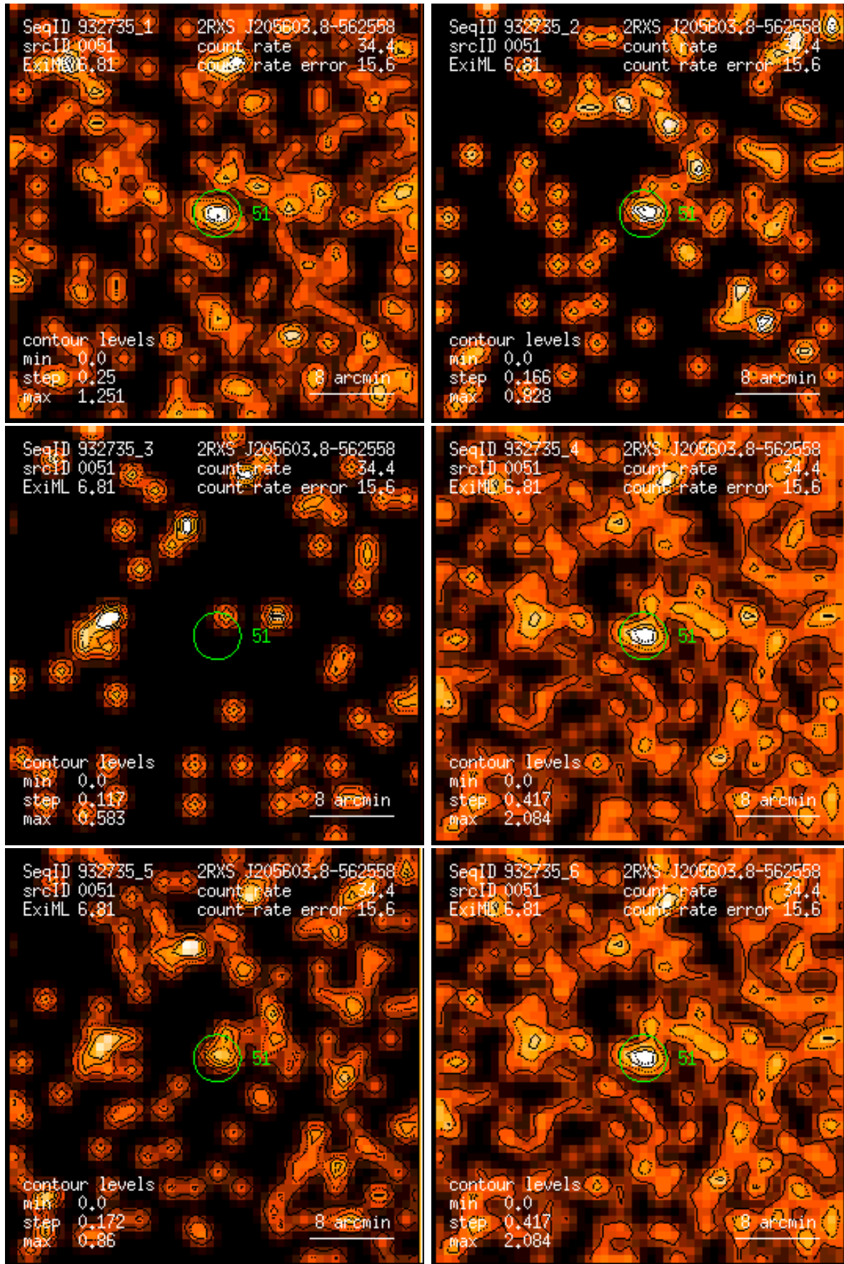
Figure 51: RASS 932735: detection 0051: band rate images, Gaussian filter: (1) PSPC channels 11 – 41, (2) 52 – 90, (3) 91 – 201, (4) 11 – 235, (5) 52 – 201, (6) 11 – 201. Broad band rates in counts/ks. Band rate contour levels in counts/ks/arcmin 2 .
