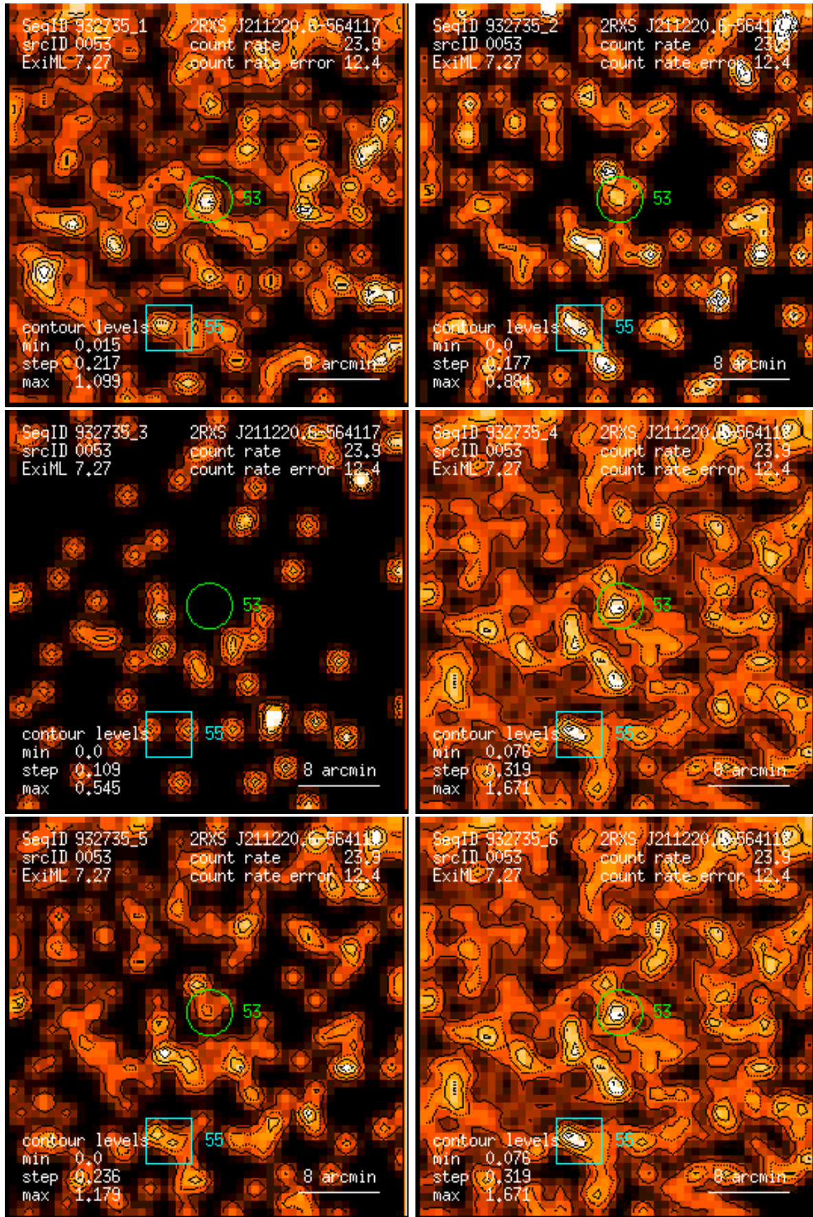
Figure 53: RASS 932735: detection 0053: band rate images, Gaussian filter: (1) PSPC channels 11 – 41, (2) 52 – 90, (3) 91 – 201, (4) 11 – 235, (5) 52 – 201, (6) 11 – 201. Broad band rates in counts/ks. Band rate contour levels in counts/ks/arcmin 2 .
