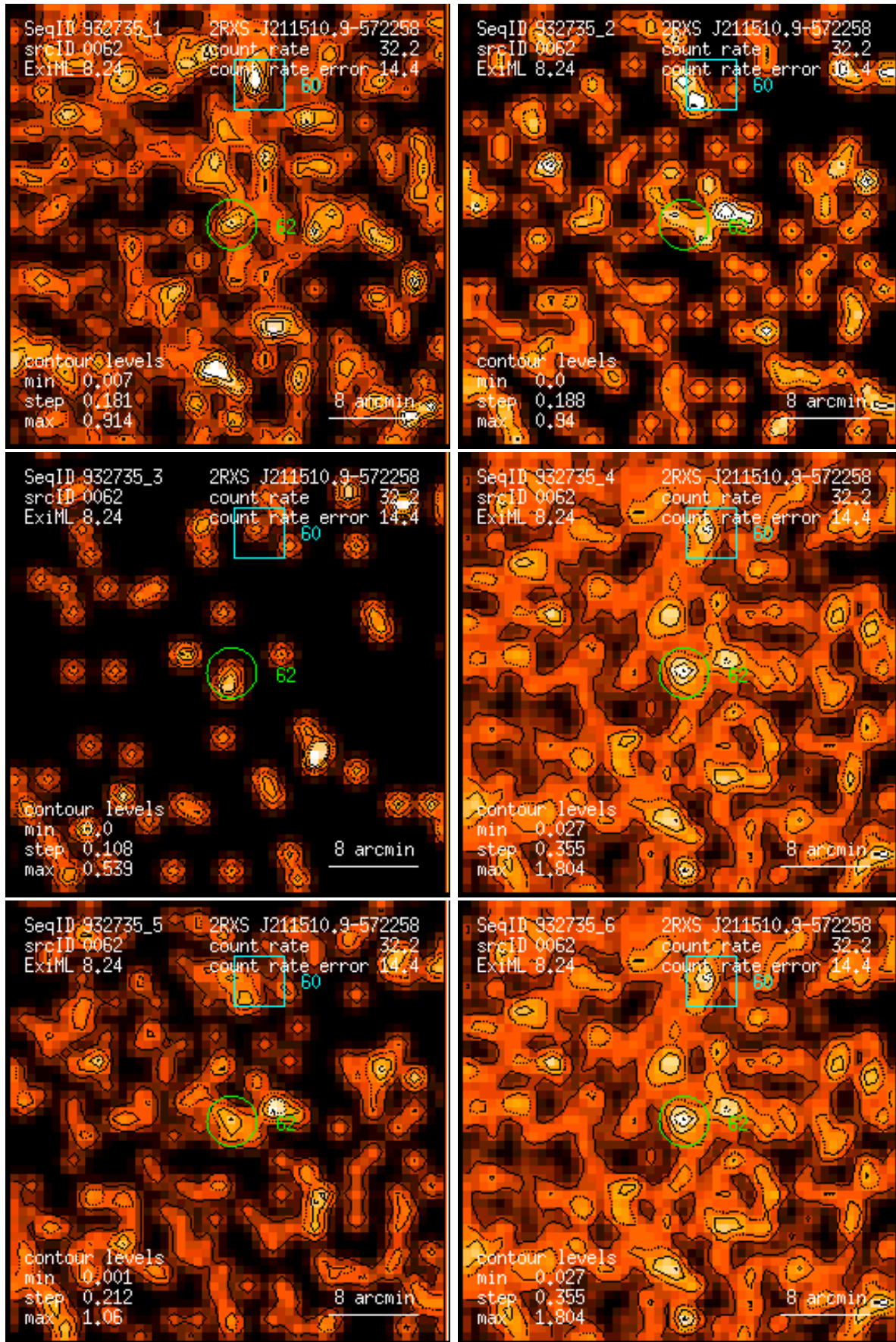
Figure 62: RASS 932735: detection 0062: band rate images, Gaussian filter: (1) PSPC channels 11 – 41, (2) 52 – 90, (3) 91 – 201, (4) 11 – 235, (5) 52 – 201, (6) 11 – 201. Broad band rates in counts/ks. Band rate contour levels in counts/ks/arcmin 2 .
