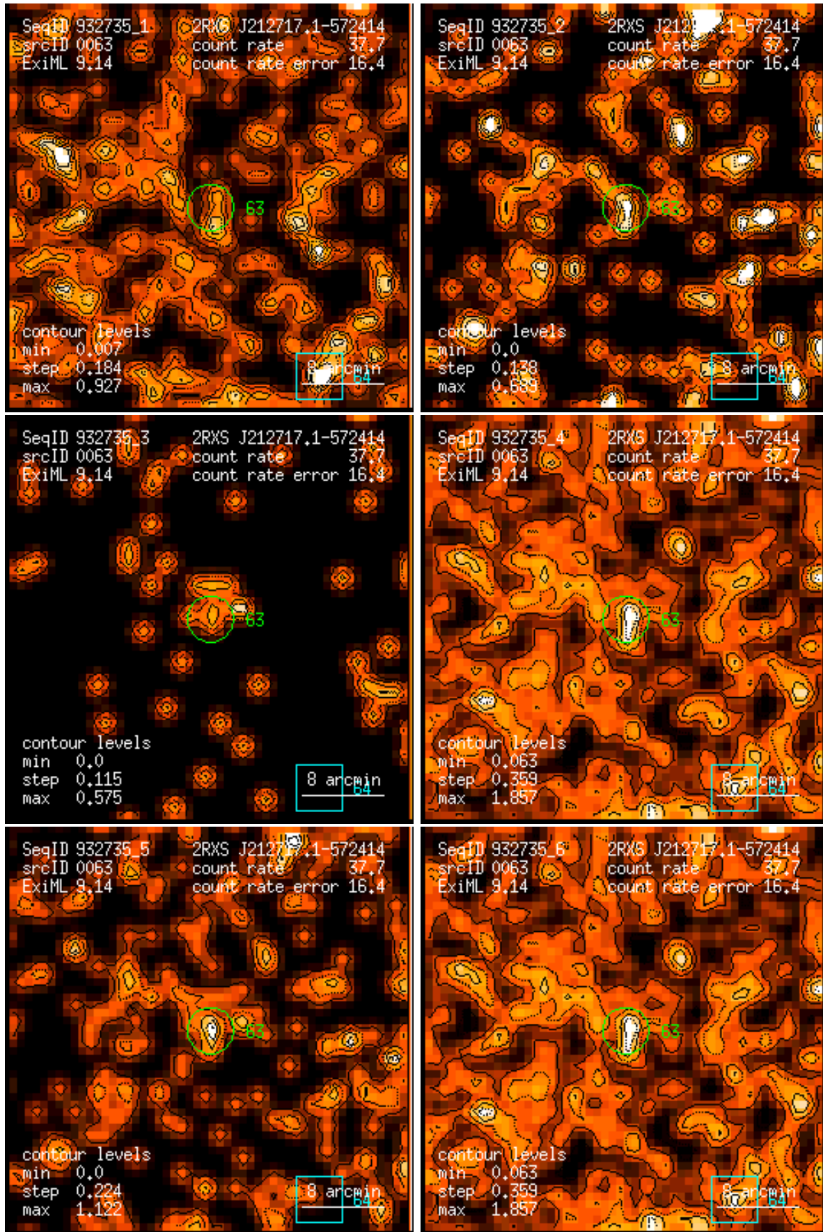
Figure 63: RASS 932735: detection 0063: band rate images, Gaussian filter: (1) PSPC channels 11 – 41, (2) 52 – 90, (3) 91 – 201, (4) 11 – 235, (5) 52 – 201, (6) 11 – 201. Broad band rates in counts/ks. Band rate contour levels in counts/ks/arcmin 2 .
