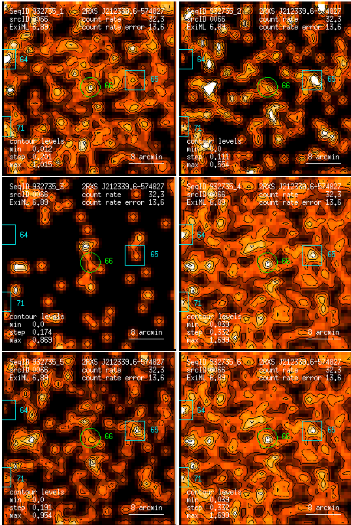
Figure 66: RASS 932735: detection 0066: band rate images, Gaussian filter: (1) PSPC channels 11 – 41, (2) 52 – 90, (3) 91 – 201, (4) 11 – 235, (5) 52 – 201, (6) 11 – 201. Broad band rates in counts/ks. Band rate contour levels in counts/ks/arcmin 2 .
