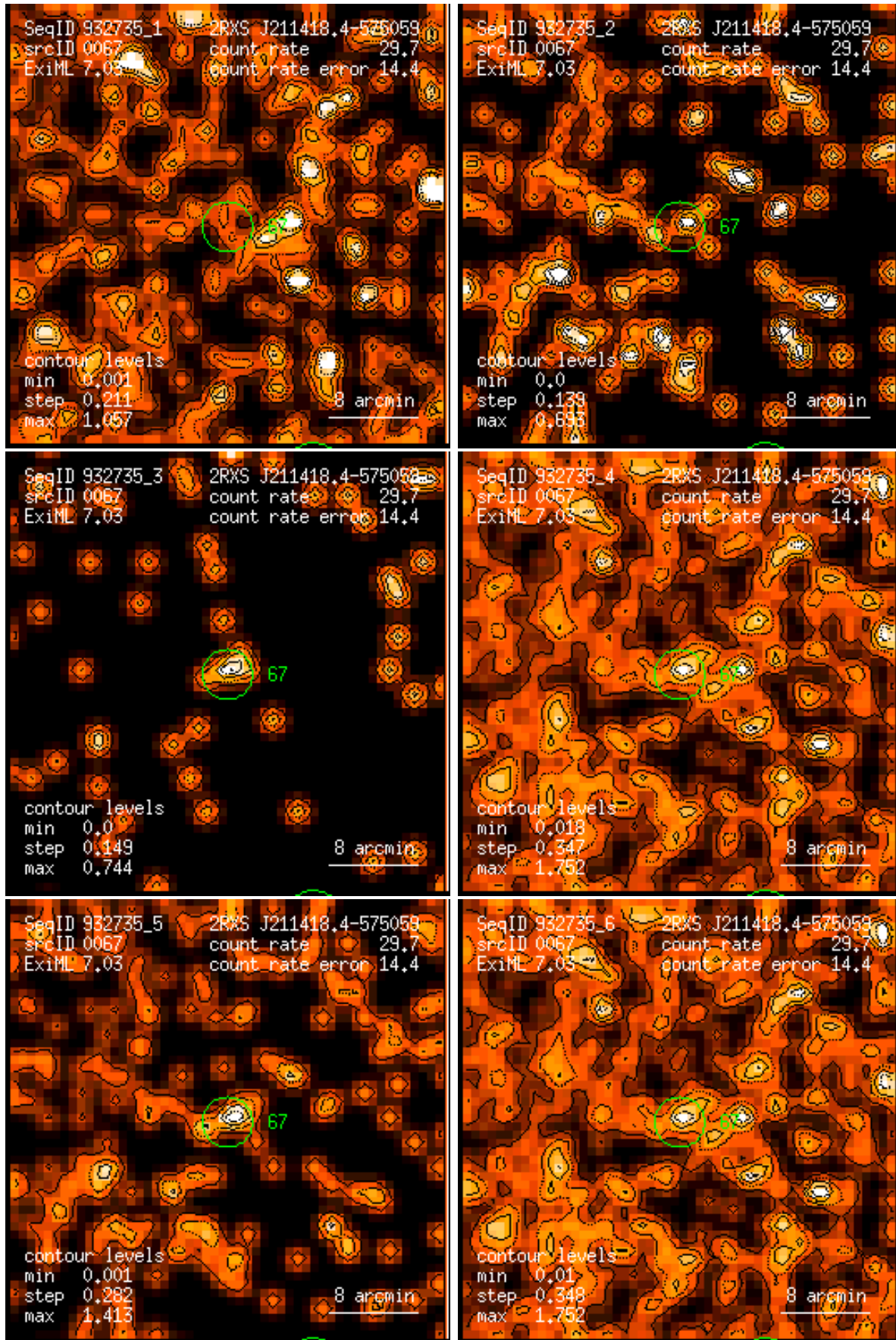
Figure 67: RASS 932735: detection 0067: band rate images, Gaussian filter: (1) PSPC channels 11 – 41, (2) 52 – 90, (3) 91 – 201, (4) 11 – 235, (5) 52 – 201, (6) 11 – 201. Broad band rates in counts/ks. Band rate contour levels in counts/ks/arcmin 2 .
