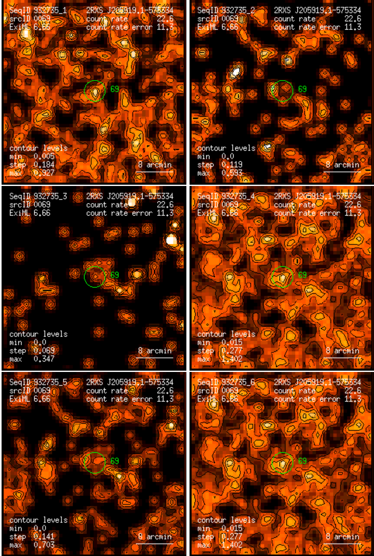
Figure 69: RASS 932735: detection 0069: band rate images, Gaussian filter: (1) PSPC channels 11 – 41, (2) 52 – 90, (3) 91 – 201, (4) 11 – 235, (5) 52 – 201, (6) 11 – 201. Broad band rates in counts/ks. Band rate contour levels in counts/ks/arcmin 2 .
