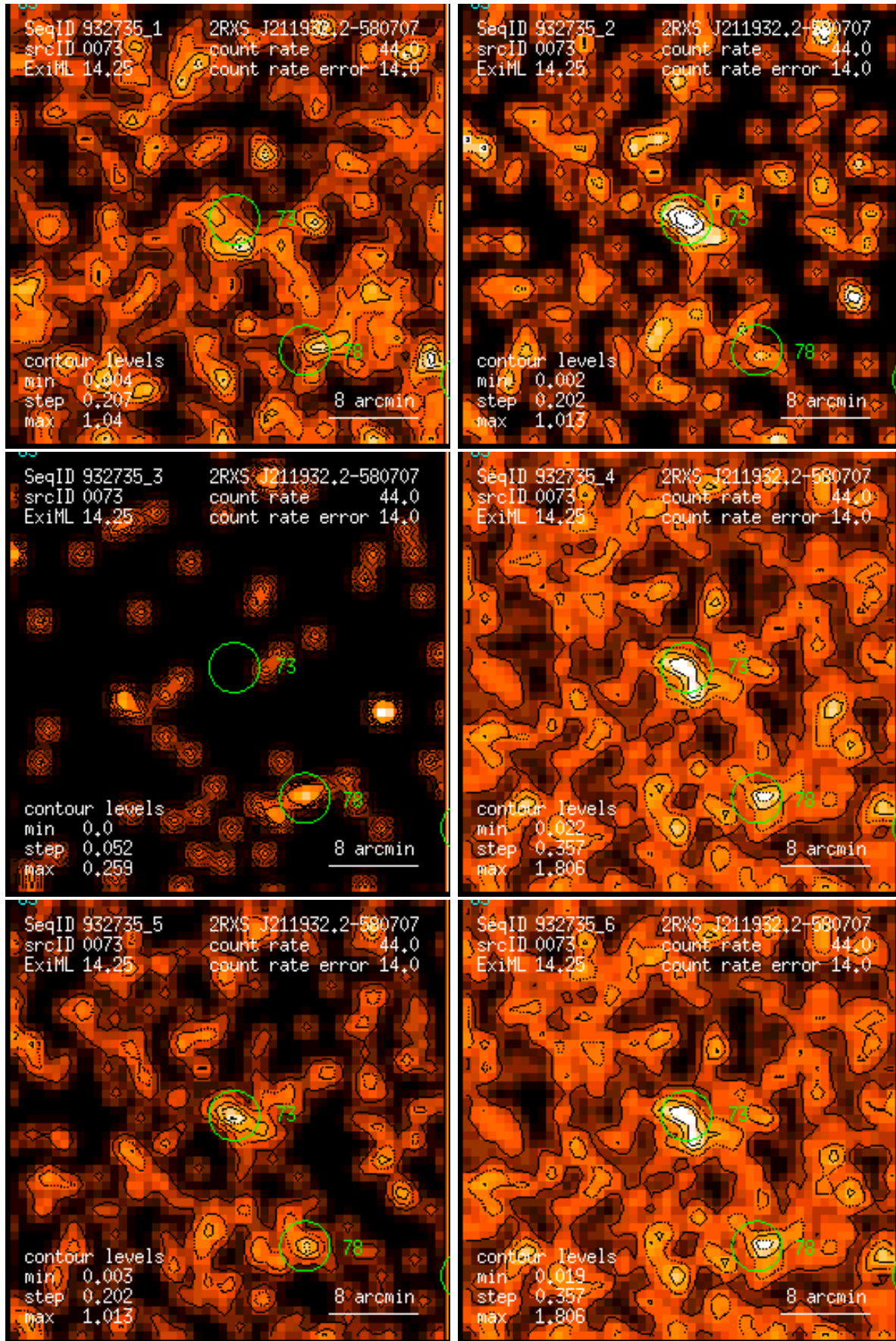
Figure 73: RASS 932735: detection 0073: band rate images, Gaussian filter: (1) PSPC channels 11 – 41, (2) 52 – 90, (3) 91 – 201, (4) 11 – 235, (5) 52 – 201, (6) 11 – 201. Broad band rates in counts/ks. Band rate contour levels in counts/ks/arcmin 2 .
