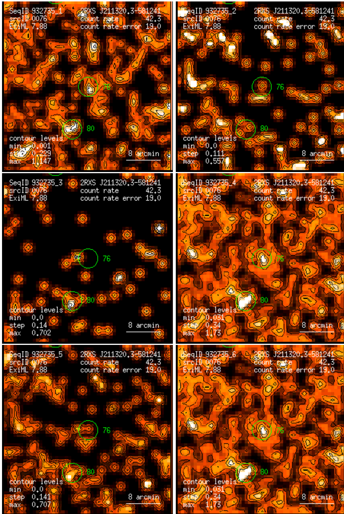
Figure 76: RASS 932735: detection 0076: band rate images, Gaussian filter: (1) PSPC channels 11 – 41, (2) 52 – 90, (3) 91 – 201, (4) 11 – 235, (5) 52 – 201, (6) 11 – 201. Broad band rates in counts/ks. Band rate contour levels in counts/ks/arcmin 2 .
