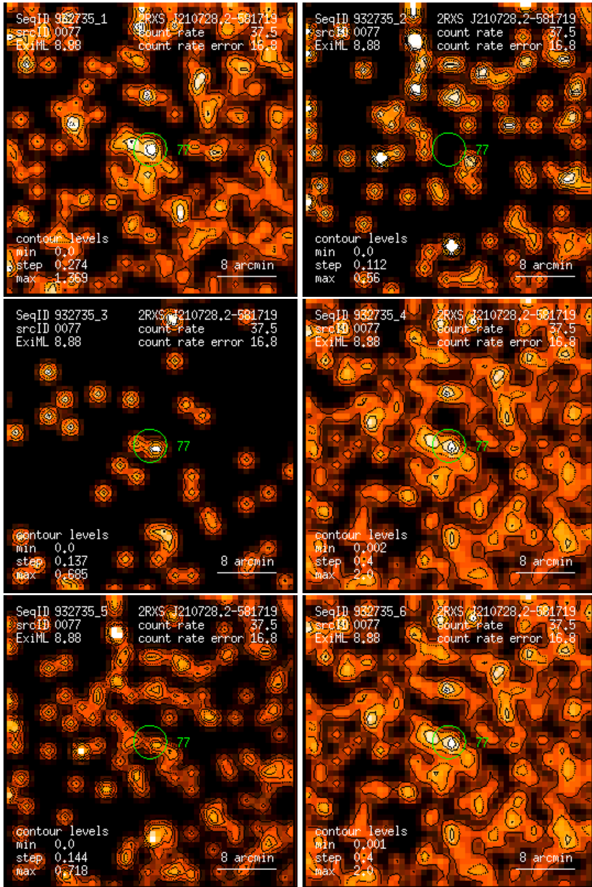
Figure 77: RASS 932735: detection 0077: band rate images, Gaussian filter: (1) PSPC channels 11 – 41, (2) 52 – 90, (3) 91 – 201, (4) 11 – 235, (5) 52 – 201, (6) 11 – 201. Broad band rates in counts/ks. Band rate contour levels in counts/ks/arcmin 2 .
