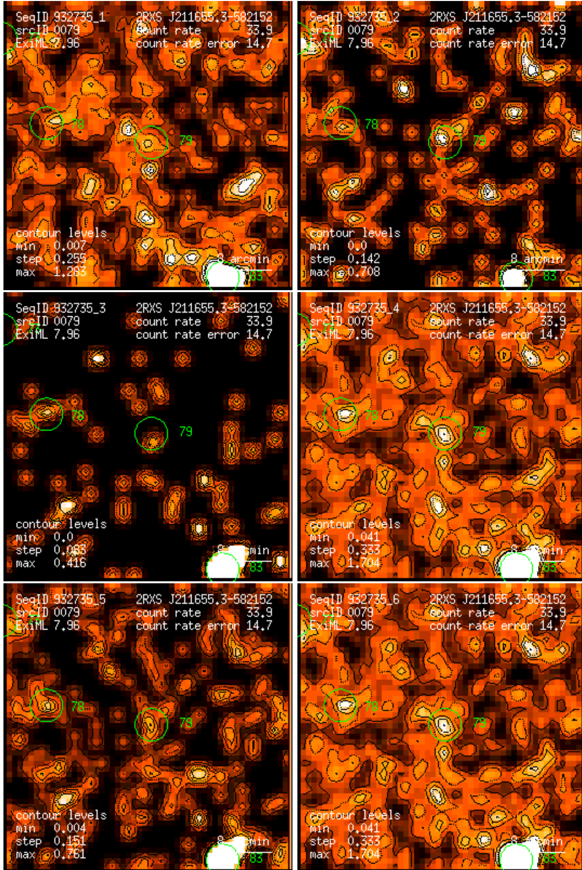
Figure 79: RASS 932735: detection 0079: band rate images, Gaussian filter: (1) PSPC channels 11 – 41, (2) 52 – 90, (3) 91 – 201, (4) 11 – 235, (5) 52 – 201, (6) 11 – 201. Broad band rates in counts/ks. Band rate contour levels in counts/ks/arcmin 2 .
