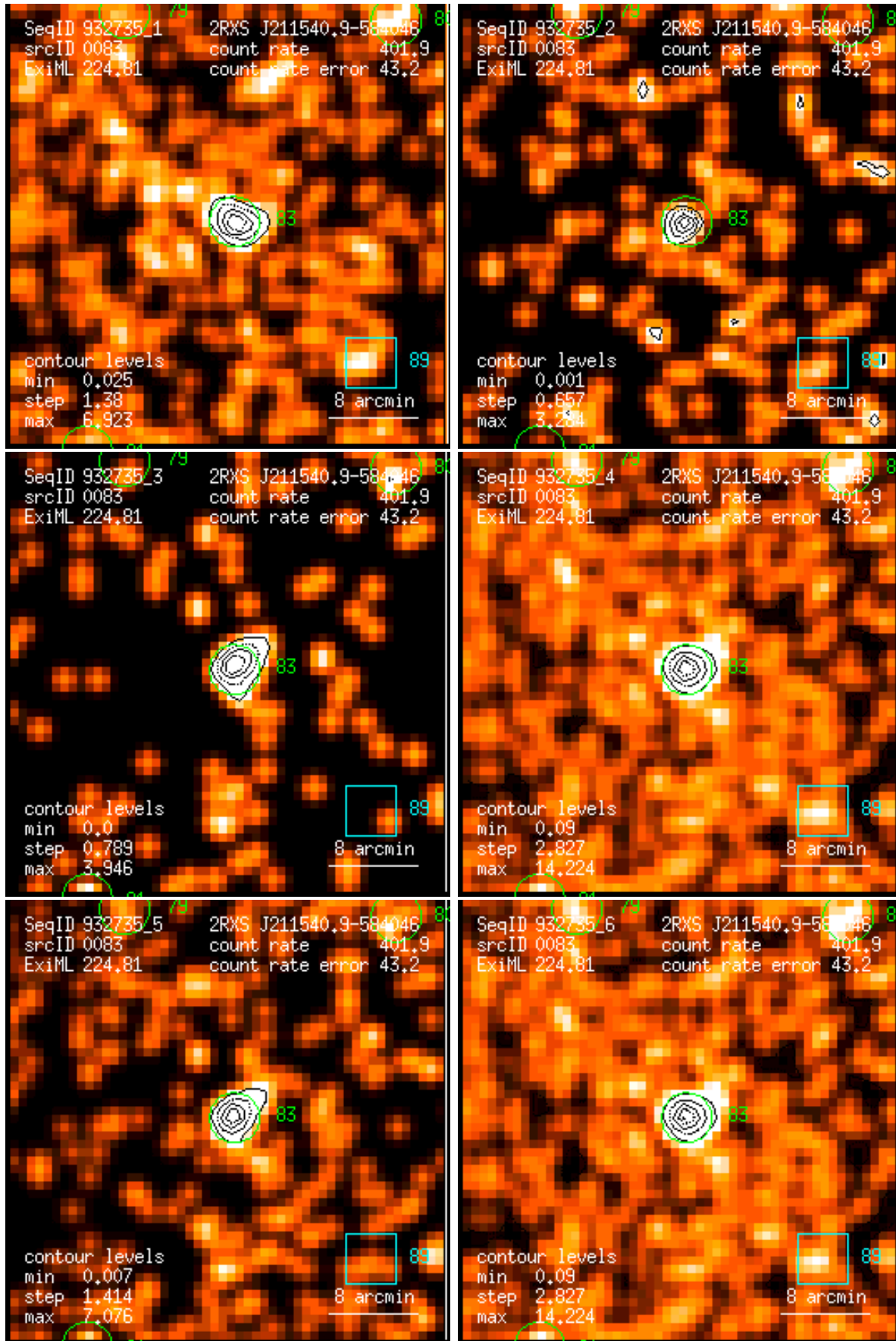
Figure 83: RASS 932735: detection 0083: band rate images, Gaussian filter: (1) PSPC channels 11 – 41, (2) 52 – 90, (3) 91 – 201, (4) 11 – 235, (5) 52 – 201, (6) 11 – 201. Broad band rates in counts/ks. Band rate contour levels in counts/ks/arcmin 2 .
