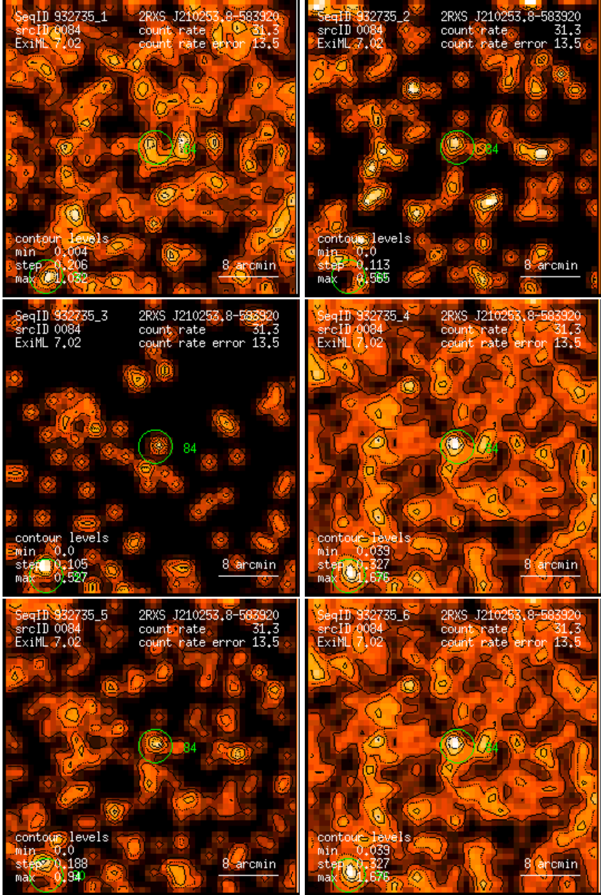
Figure 84: RASS 932735: detection 0084: band rate images, Gaussian filter: (1) PSPC channels 11 – 41, (2) 52 – 90, (3) 91 – 201, (4) 11 – 235, (5) 52 – 201, (6) 11 – 201. Broad band rates in counts/ks. Band rate contour levels in counts/ks/arcmin 2 .
