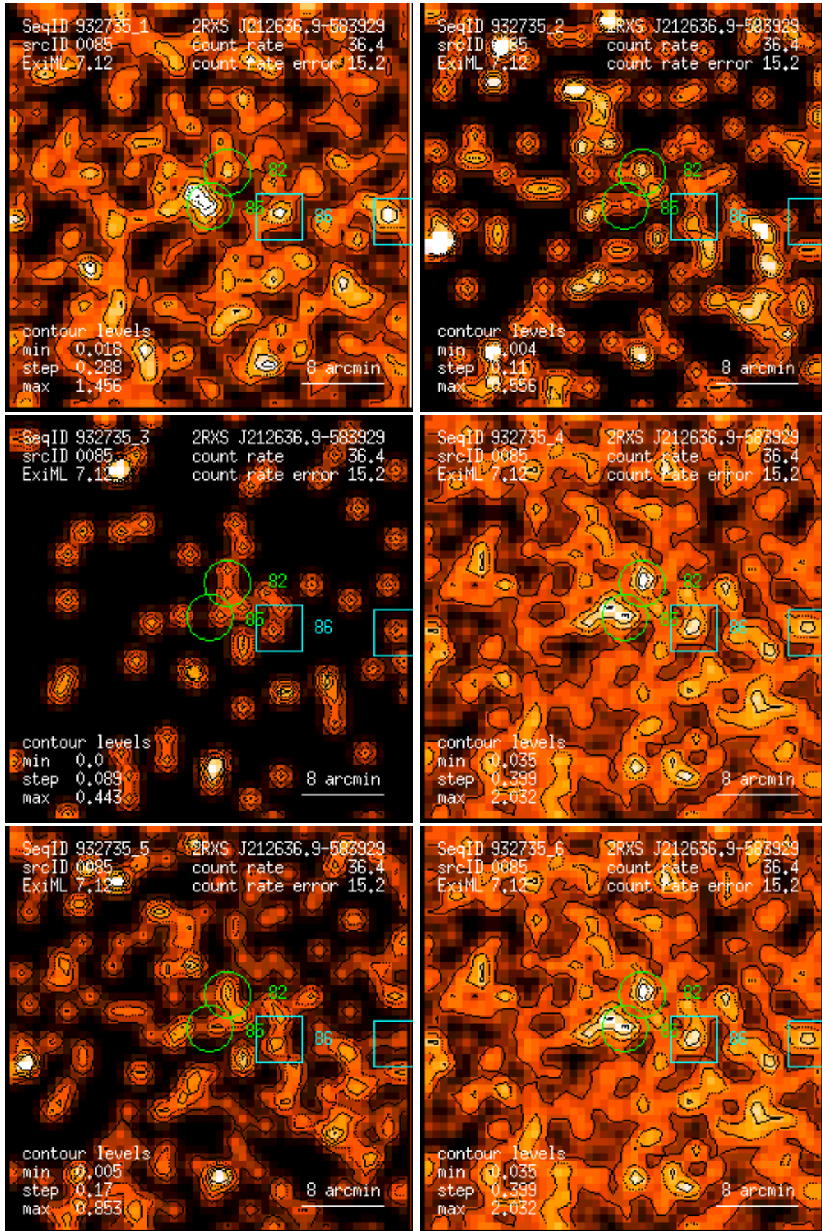
Figure 85: RASS 932735: detection 0085: band rate images, Gaussian filter: (1) PSPC channels 11 – 41, (2) 52 – 90, (3) 91 – 201, (4) 11 – 235, (5) 52 – 201, (6) 11 – 201. Broad band rates in counts/ks. Band rate contour levels in counts/ks/arcmin 2 .
