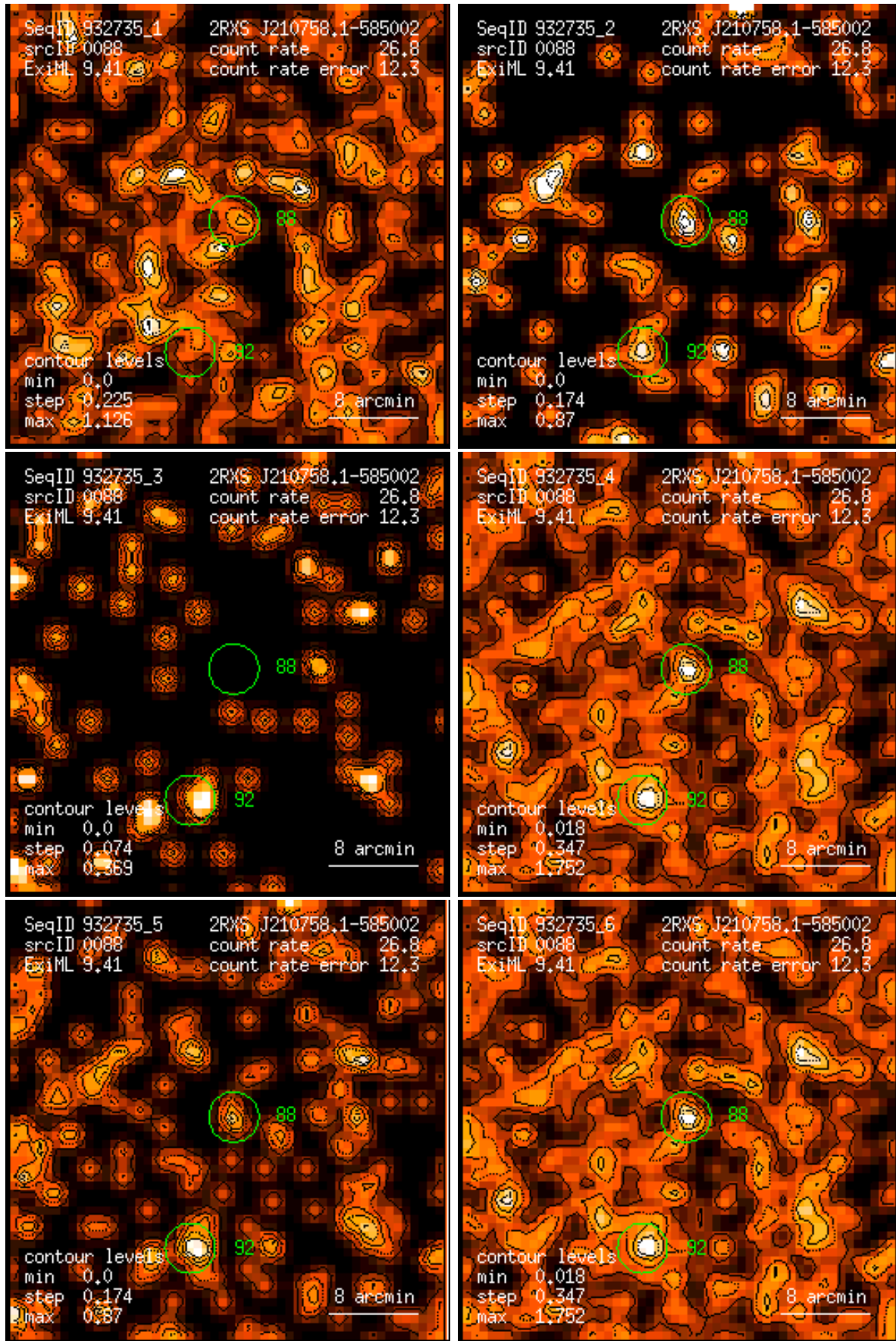
Figure 88: RASS 932735: detection 0088: band rate images, Gaussian filter: (1) PSPC channels 11 – 41, (2) 52 – 90, (3) 91 – 201, (4) 11 – 235, (5) 52 – 201, (6) 11 – 201. Broad band rates in counts/ks. Band rate contour levels in counts/ks/arcmin 2 .
