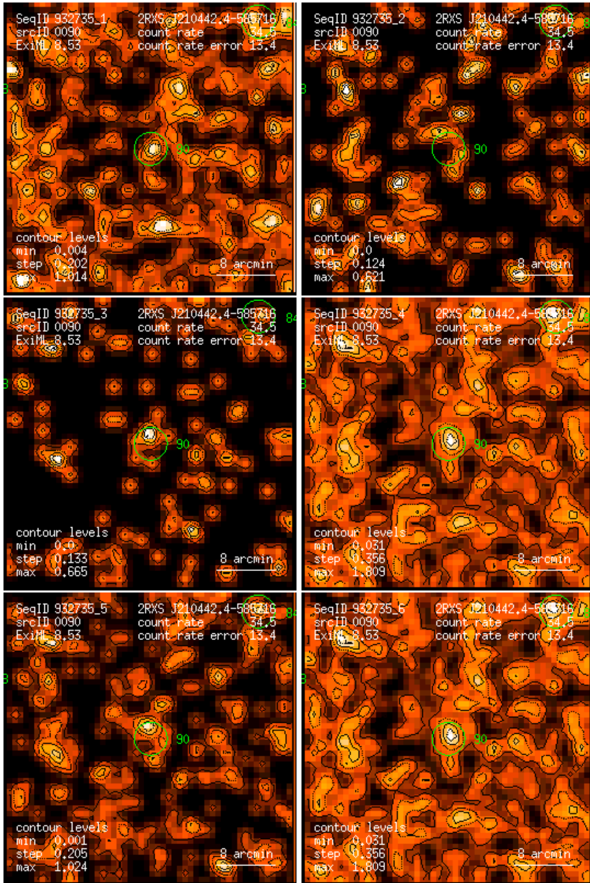
Figure 90: RASS 932735: detection 0090: band rate images, Gaussian filter: (1) PSPC channels 11 – 41, (2) 52 – 90, (3) 91 – 201, (4) 11 – 235, (5) 52 – 201, (6) 11 – 201. Broad band rates in counts/ks. Band rate contour levels in counts/ks/arcmin 2 .
