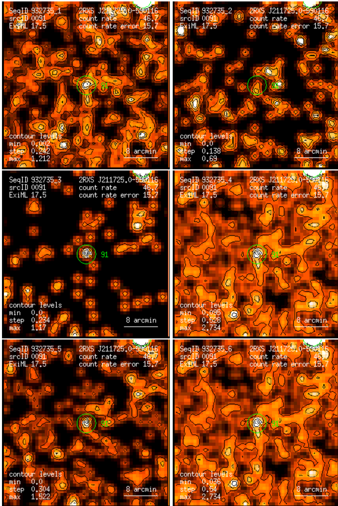
Figure 91: RASS 932735: detection 0091: band rate images, Gaussian filter: (1) PSPC channels 11 – 41, (2) 52 – 90, (3) 91 – 201, (4) 11 – 235, (5) 52 – 201, (6) 11 – 201. Broad band rates in counts/ks. Band rate contour levels in counts/ks/arcmin 2 .
