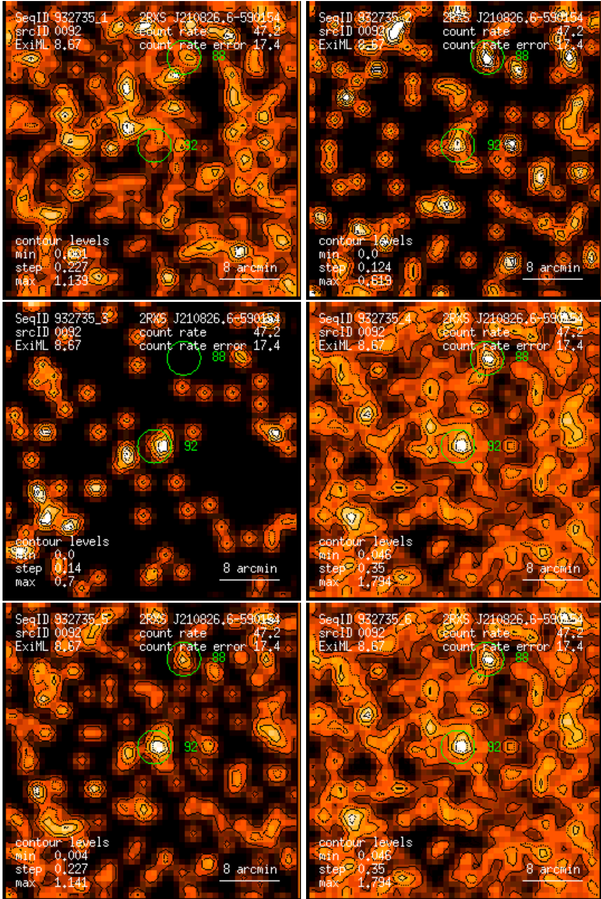
Figure 92: RASS 932735: detection 0092: band rate images, Gaussian filter: (1) PSPC channels 11 – 41, (2) 52 – 90, (3) 91 – 201, (4) 11 – 235, (5) 52 – 201, (6) 11 – 201. Broad band rates in counts/ks. Band rate contour levels in counts/ks/arcmin 2 .
