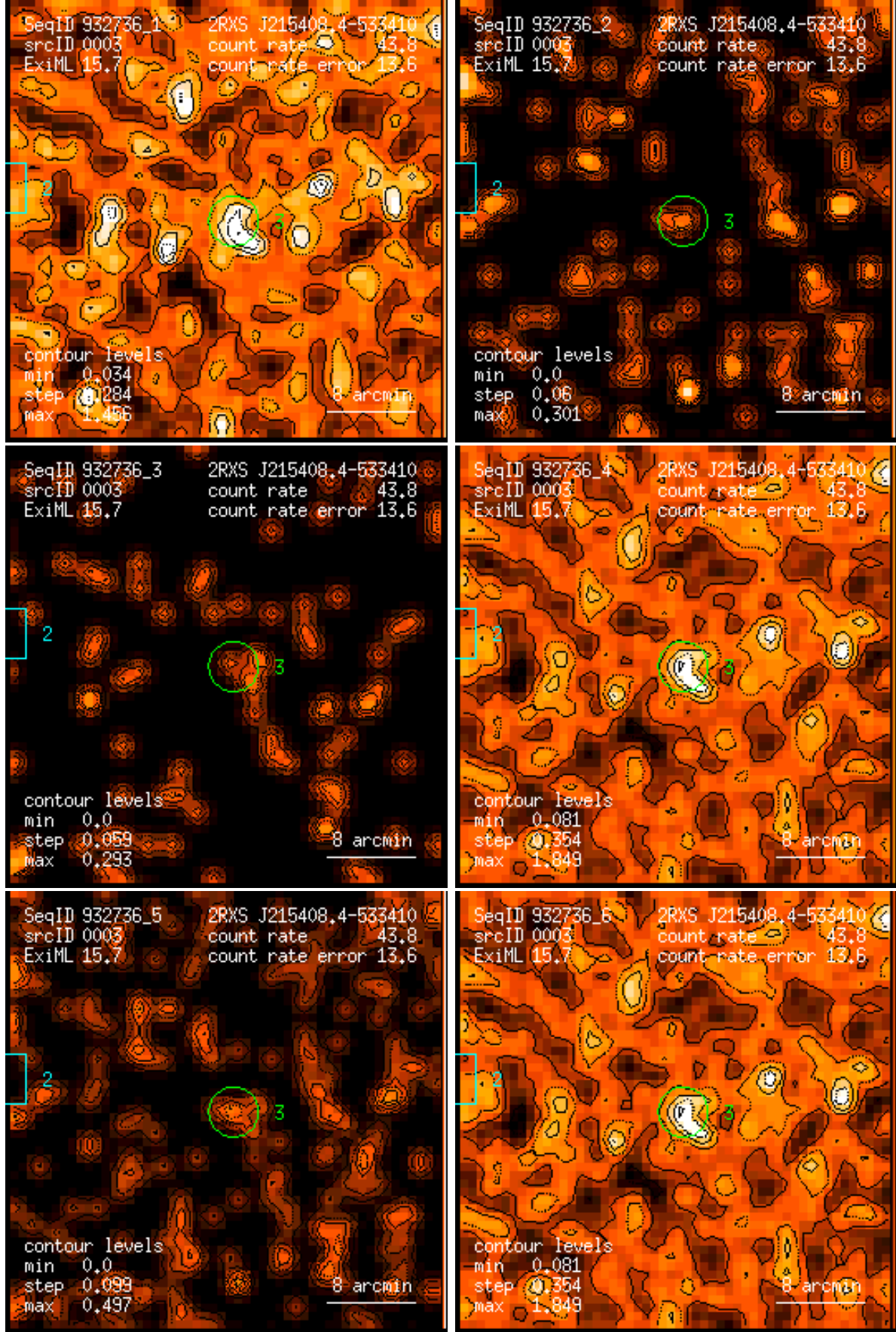
Figure 3: RASS 932736: detection 0003: band rate images, Gaussian filter: (1) PSPC channels 11 – 41, (2) 52 – 90, (3) 91 – 201, (4) 11 – 235, (5) 52 – 201, (6) 11 – 201. Broad band rates in counts/ks. Band rate contour levels in counts/ks/arcmin 2 .
