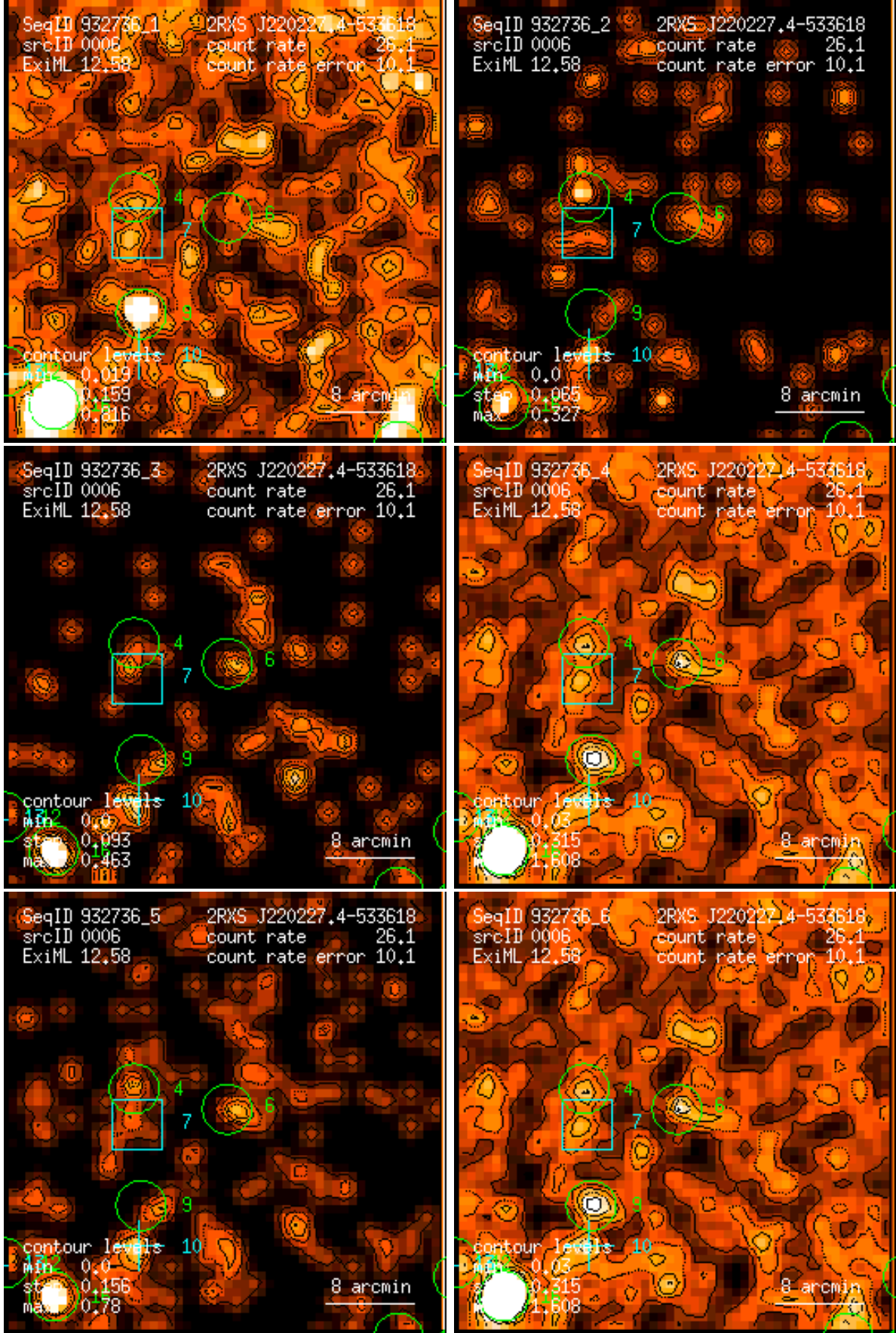
Figure 6: RASS 932736: detection 0006: band rate images, Gaussian filter: (1) PSPC channels 11 – 41, (2) 52 – 90, (3) 91 – 201, (4) 11 – 235, (5) 52 – 201, (6) 11 – 201. Broad band rates in counts/ks. Band rate contour levels in counts/ks/arcmin 2 .
