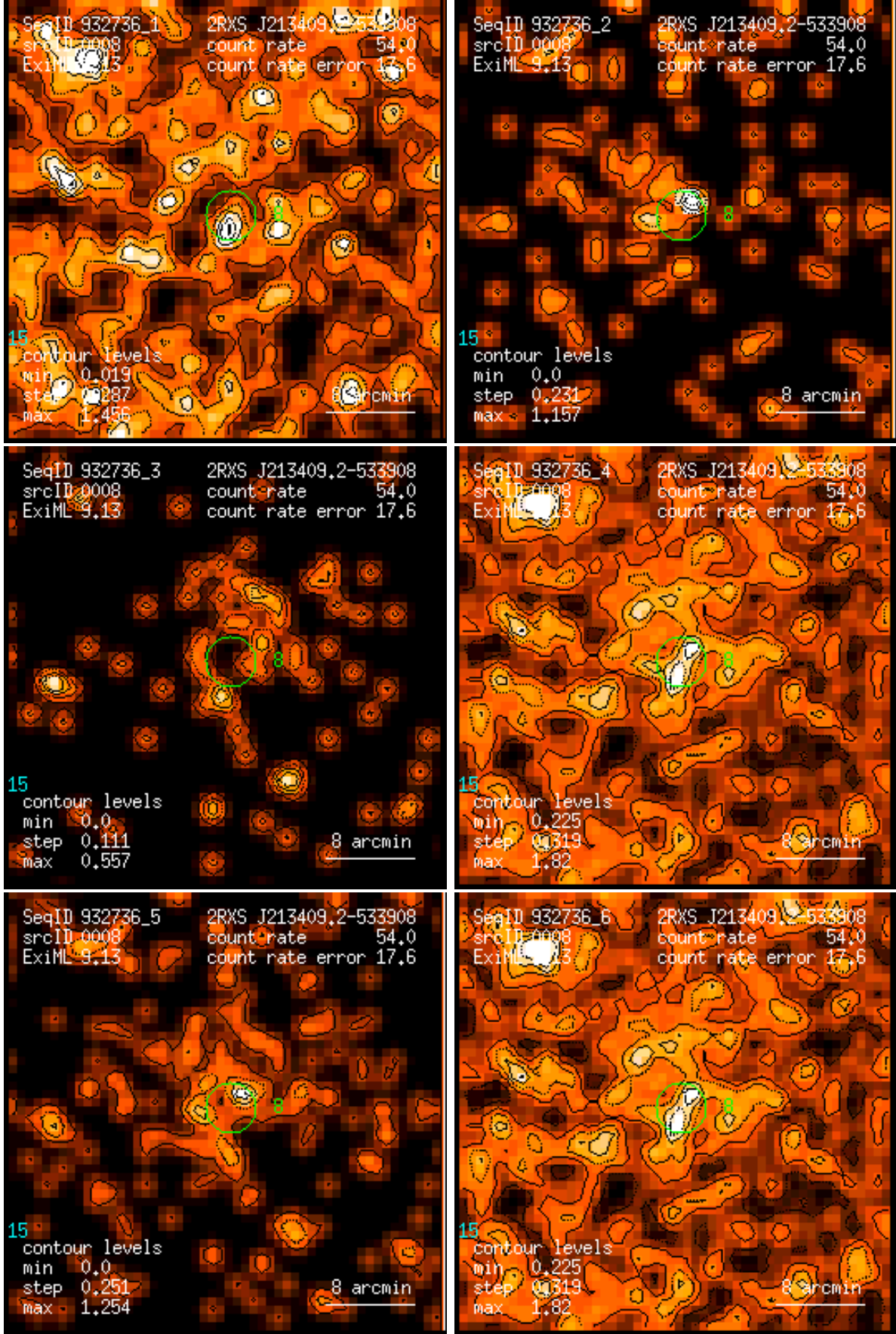
Figure 8: RASS 932736: detection 0008: band rate images, Gaussian filter: (1) PSPC channels 11 – 41, (2) 52 – 90, (3) 91 – 201, (4) 11 – 235, (5) 52 – 201, (6) 11 – 201. Broad band rates in counts/ks. Band rate contour levels in counts/ks/arcmin 2 .
