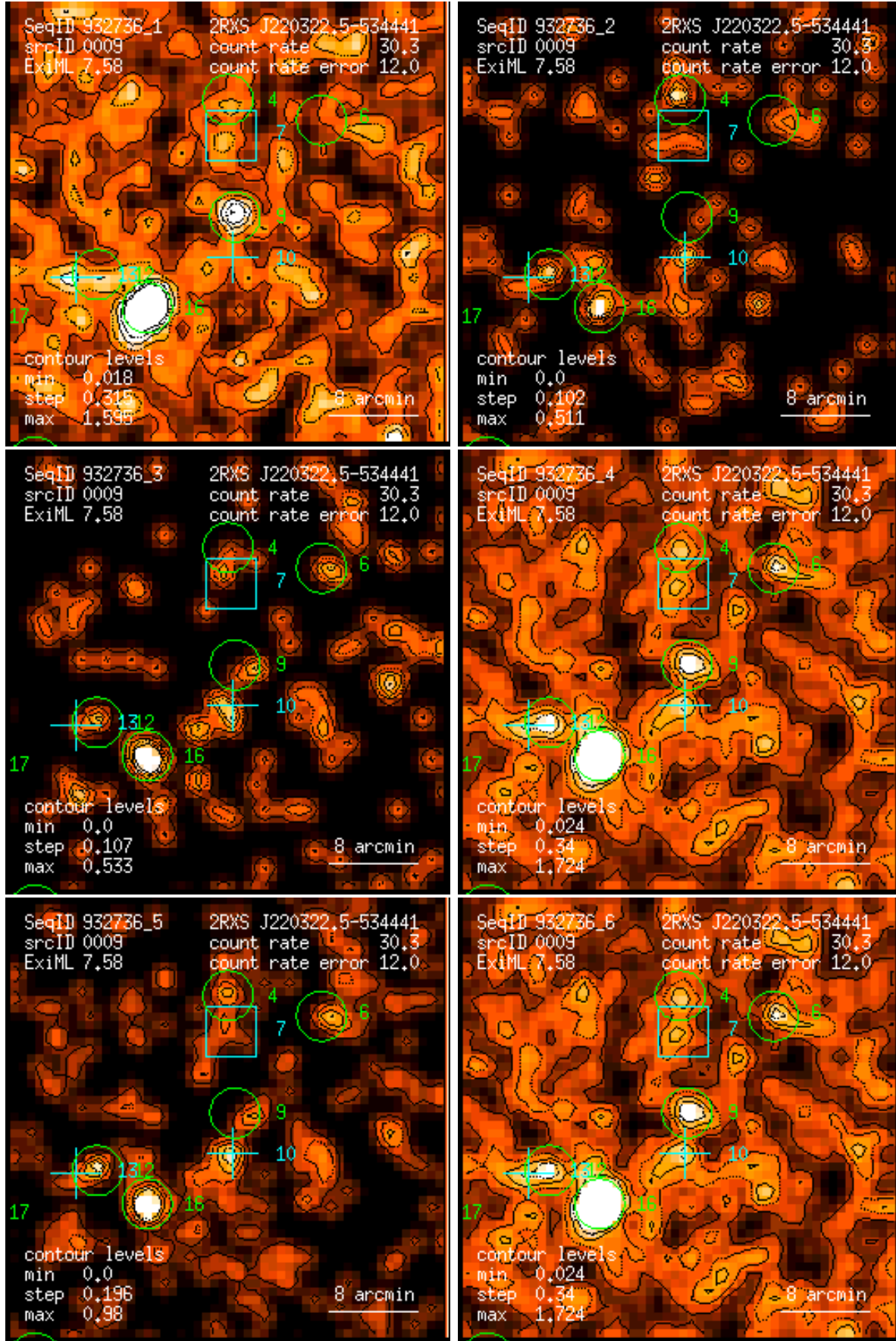
Figure 9: RASS 932736: detection 0009: band rate images, Gaussian filter: (1) PSPC channels 11 – 41, (2) 52 – 90, (3) 91 – 201, (4) 11 – 235, (5) 52 – 201, (6) 11 – 201. Broad band rates in counts/ks. Band rate contour levels in counts/ks/arcmin 2 .
