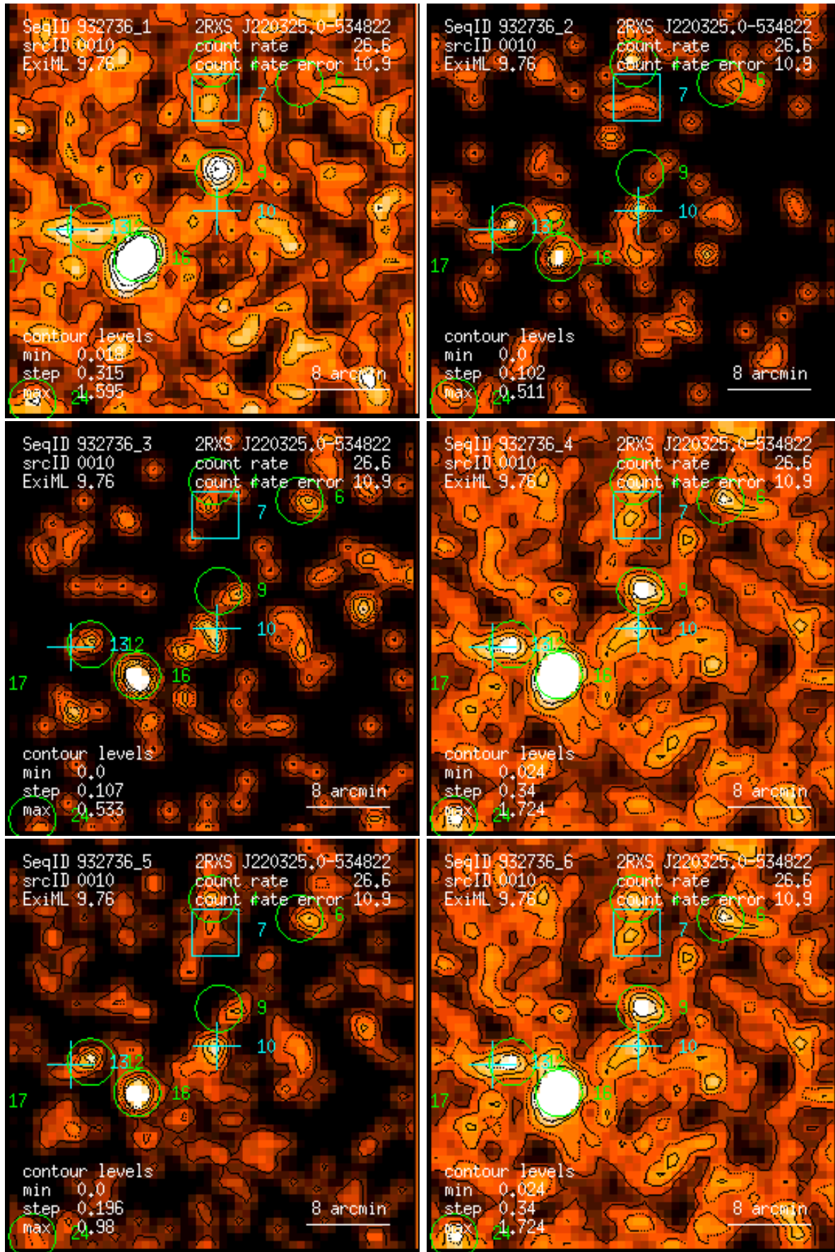
Figure 10: RASS 932736: detection 0010: band rate images, Gaussian filter: (1) PSPC channels 11 – 41, (2) 52 – 90, (3) 91 – 201, (4) 11 – 235, (5) 52 – 201, (6) 11 – 201. Broad band rates in counts/ks. Band rate contour levels in counts/ks/arcmin 2 .
