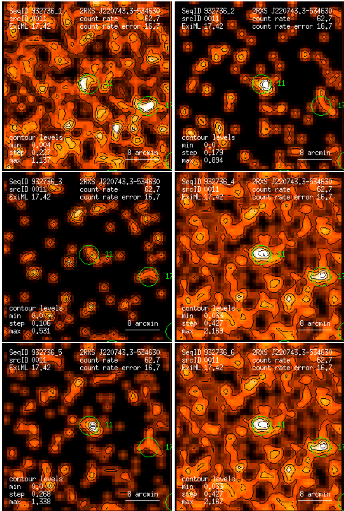
Figure 11: RASS 932736: detection 0011: band rate images, Gaussian filter: (1) PSPC channels 11 – 41, (2) 52 – 90, (3) 91 – 201, (4) 11 – 235, (5) 52 – 201, (6) 11 – 201. Broad band rates in counts/ks. Band rate contour levels in counts/ks/arcmin 2 .
