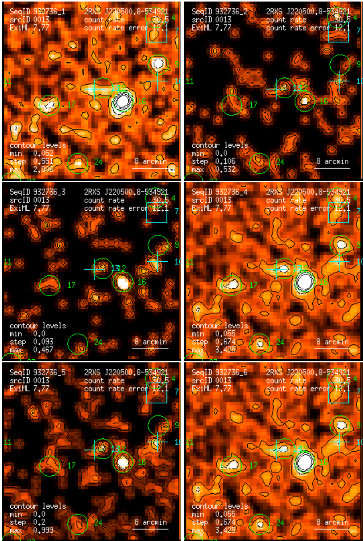
Figure 13: RASS 932736: detection 0013: band rate images, Gaussian filter: (1) PSPC channels 11 – 41, (2) 52 – 90, (3) 91 – 201, (4) 11 – 235, (5) 52 – 201, (6) 11 – 201. Broad band rates in counts/ks. Band rate contour levels in counts/ks/arcmin 2 .
