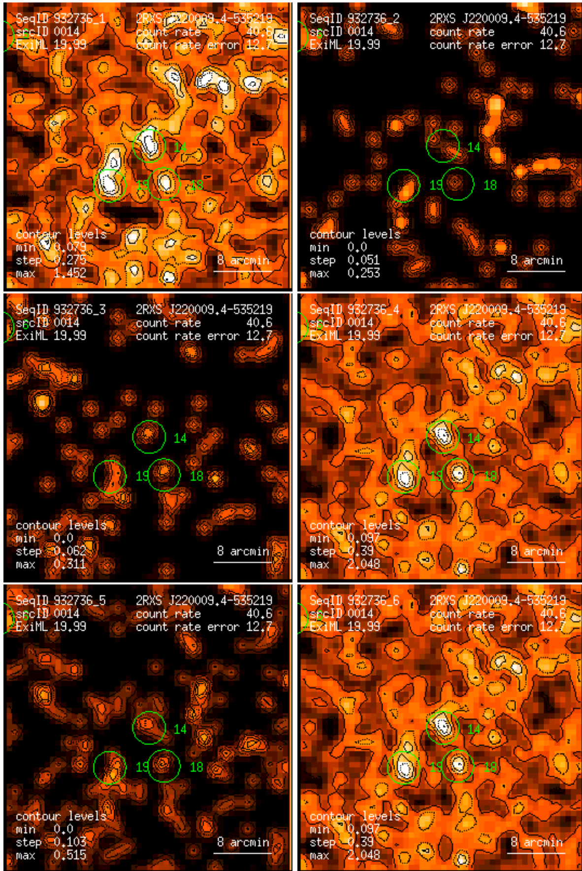
Figure 14: RASS 932736: detection 0014: band rate images, Gaussian filter: (1) PSPC channels 11 – 41, (2) 52 – 90, (3) 91 – 201, (4) 11 – 235, (5) 52 – 201, (6) 11 – 201. Broad band rates in counts/ks. Band rate contour levels in counts/ks/arcmin 2 .
