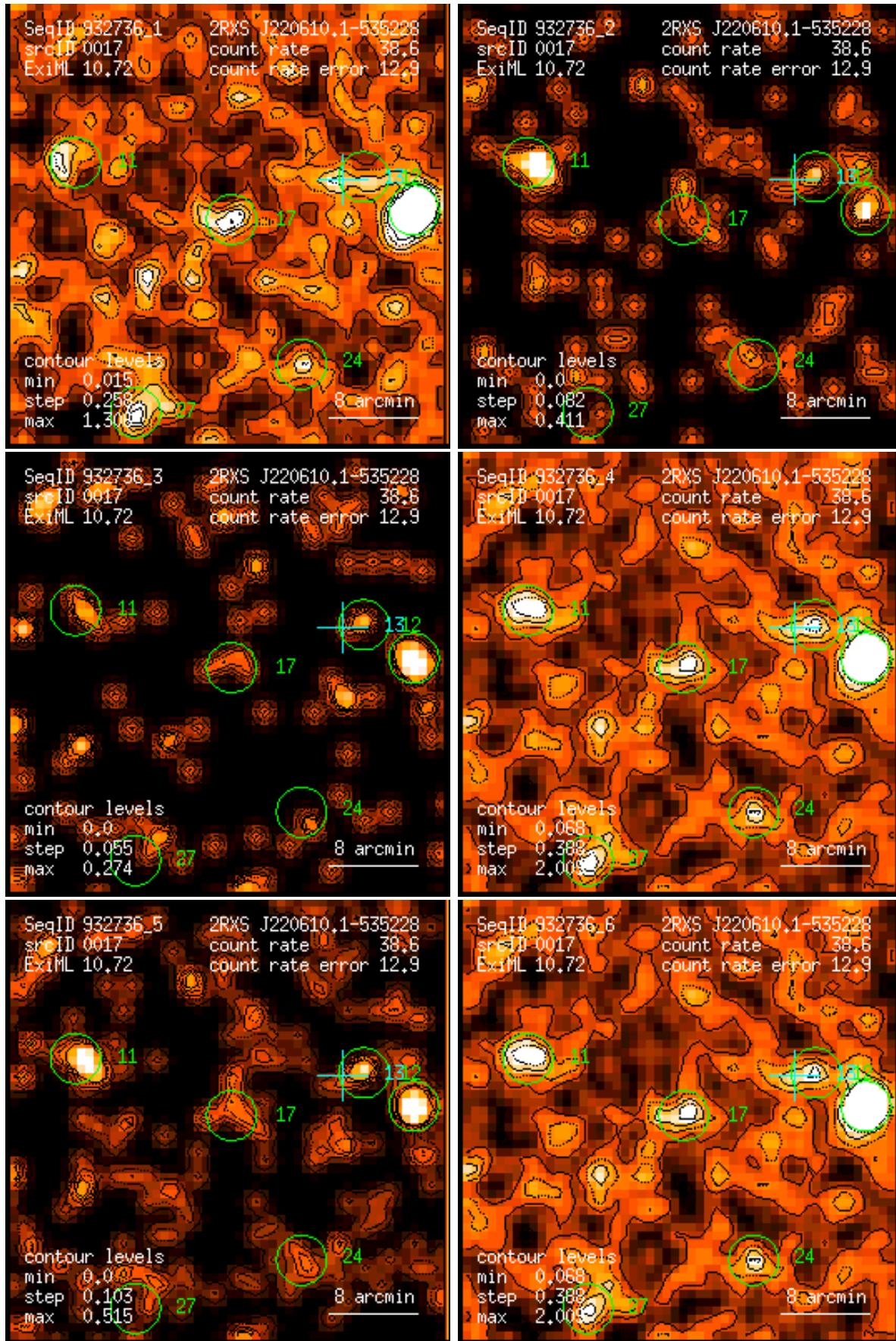
Figure 17: RASS 932736: detection 0017: band rate images, Gaussian filter: (1) PSPC channels 11 – 41, (2) 52 – 90, (3) 91 – 201, (4) 11 – 235, (5) 52 – 201, (6) 11 – 201. Broad band rates in counts/ks. Band rate contour levels in counts/ks/arcmin 2 .
