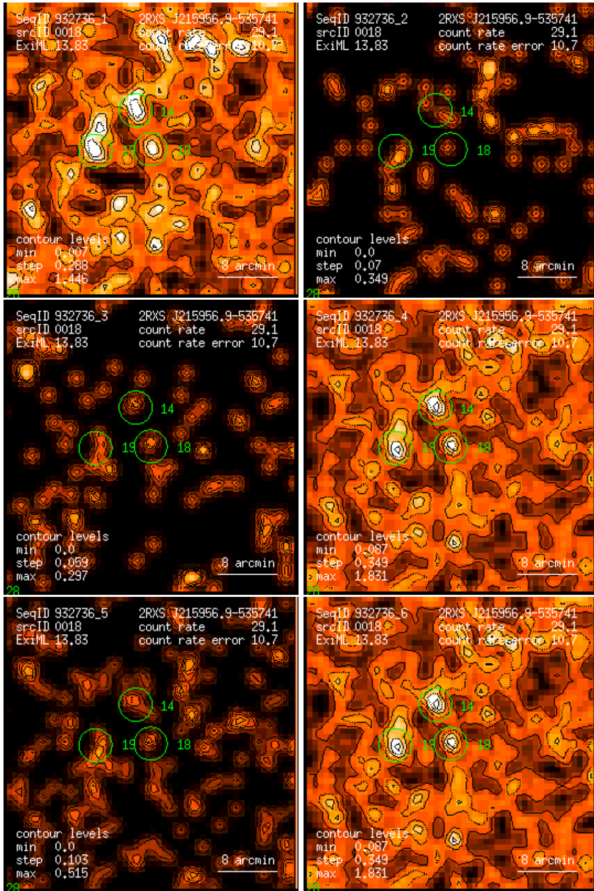
Figure 18: RASS 932736: detection 0018: band rate images, Gaussian filter: (1) PSPC channels 11 – 41, (2) 52 – 90, (3) 91 – 201, (4) 11 – 235, (5) 52 – 201, (6) 11 – 201. Broad band rates in counts/ks. Band rate contour levels in counts/ks/arcmin 2 .
