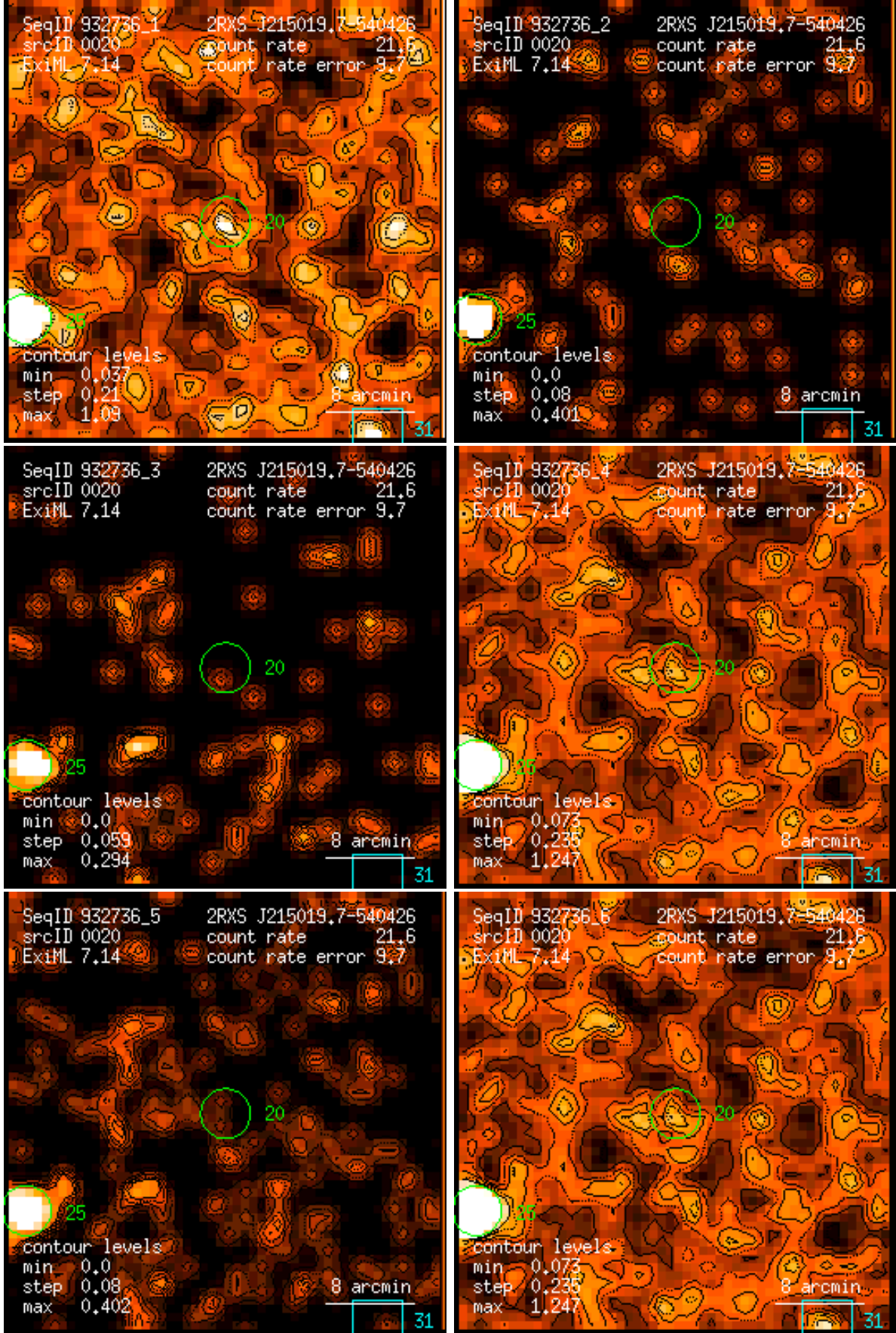
Figure 20: RASS 932736: detection 0020: band rate images, Gaussian filter: (1) PSPC channels 11 – 41, (2) 52 – 90, (3) 91 – 201, (4) 11 – 235, (5) 52 – 201, (6) 11 – 201. Broad band rates in counts/ks. Band rate contour levels in counts/ks/arcmin 2 .
