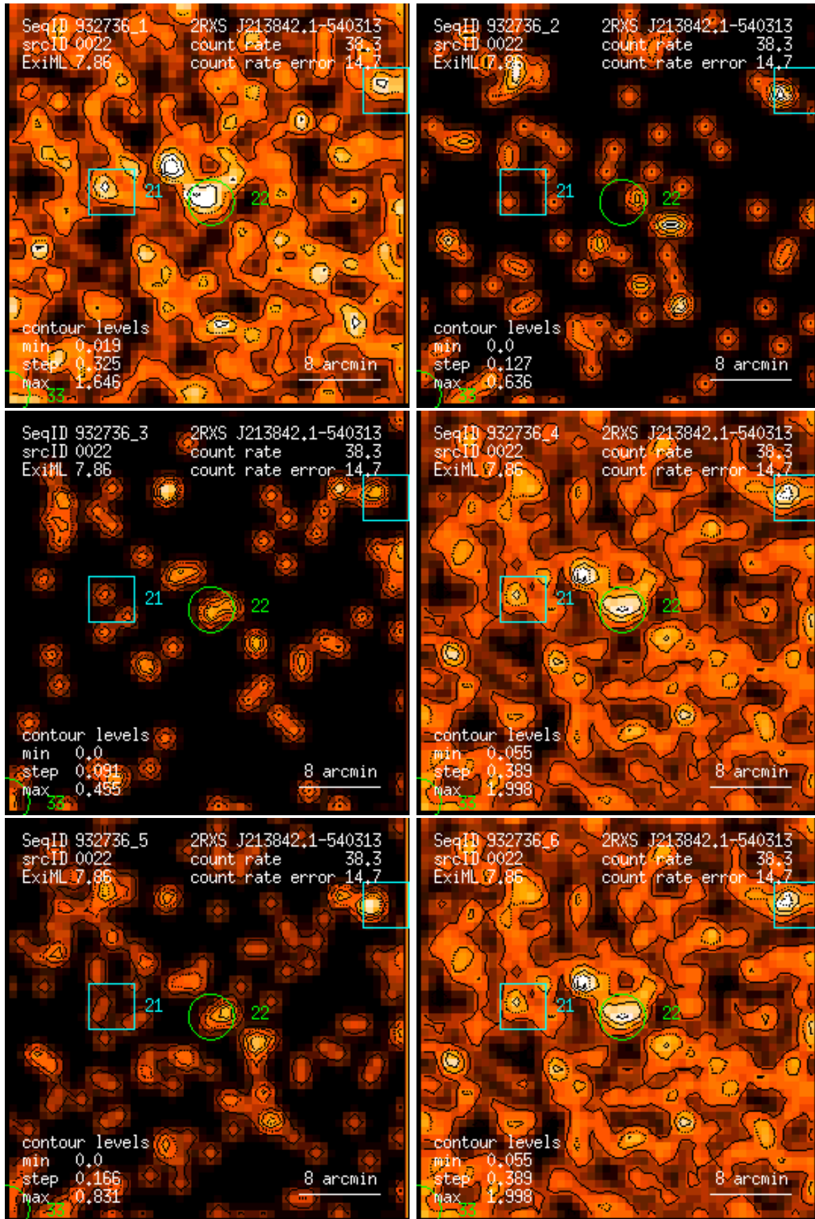
Figure 22: RASS 932736: detection 0022: band rate images, Gaussian filter: (1) PSPC channels 11 – 41, (2) 52 – 90, (3) 91 – 201, (4) 11 – 235, (5) 52 – 201, (6) 11 – 201. Broad band rates in counts/ks. Band rate contour levels in counts/ks/arcmin 2 .
